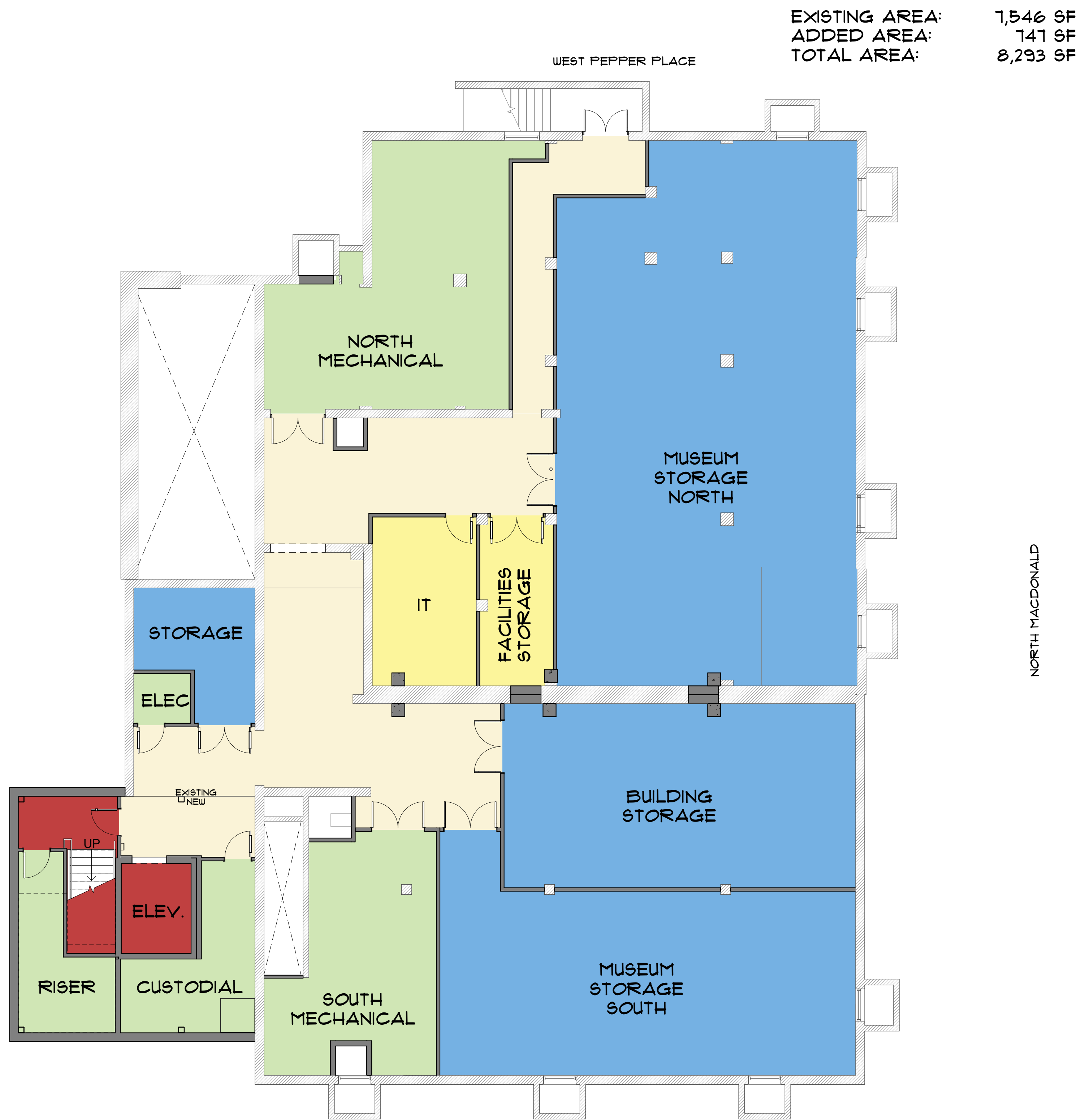
BASEMENT 1/8" = 1'-0"
