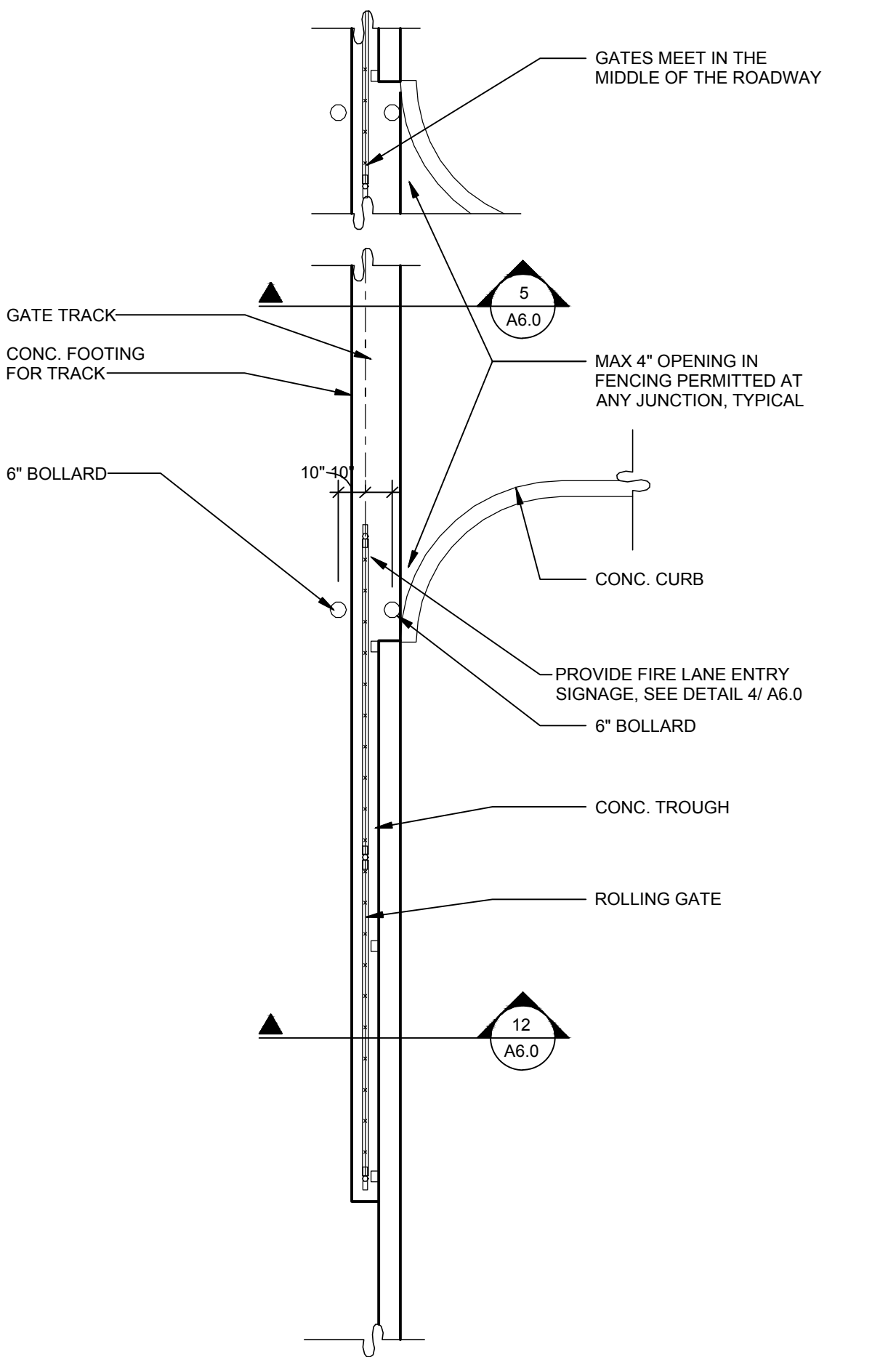
SLIDING GATE - PLAN SCALE: 1" = 1'-0"
