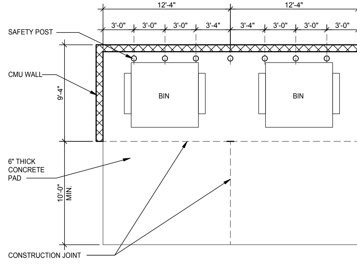
DOUBLE WIDE BIN ENCLOSURE SCALE: 3/16" = 1'-0"
