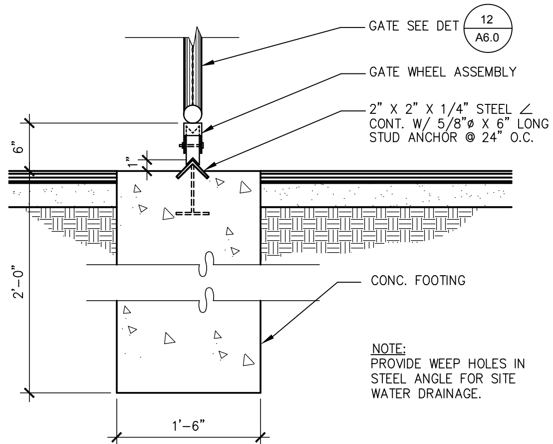
SLIDING GATE - TRACK SCALE: 3/4" = 1'-0"
