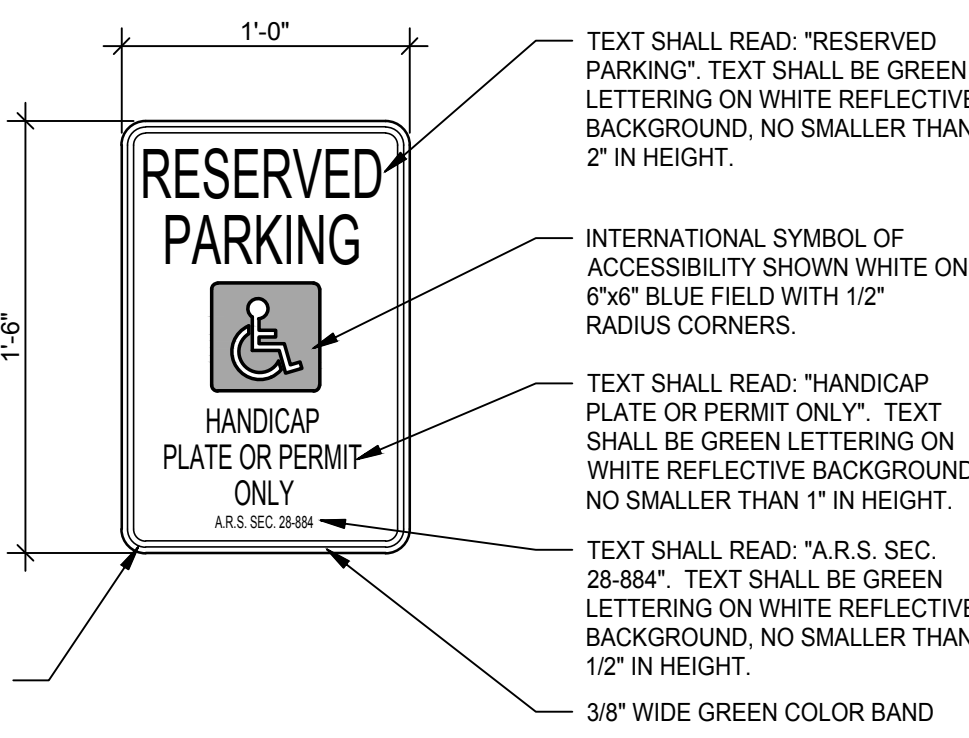
ACCESSIBLE SIGNS SCALE: 1 1/2" = 1'-0"
