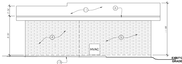
EAST ELEVATION SCALE : 3/8" = 1'- 0"
