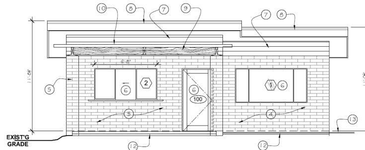
WEST ELEVATION SCALE : 3/8" = 1'- 0"
