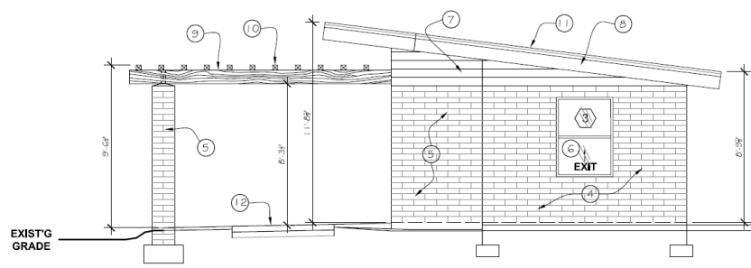
SOUTH ELEVATION SCALE : 3/8" = 1'- 0"
