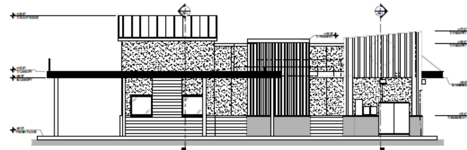
4 WEST ELEVATION
