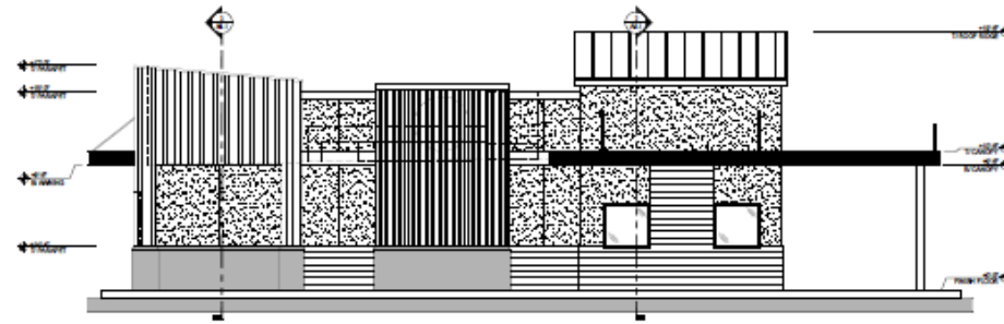
1 EAST ELEVATION
