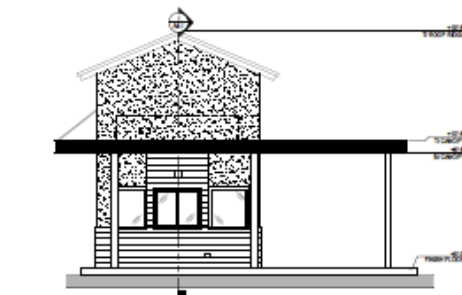
② NORTH ELEVATION
