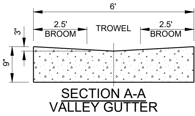
MODIFIED MAG STD DETAIL 240 VALLEY GUTTER NO SCALE
