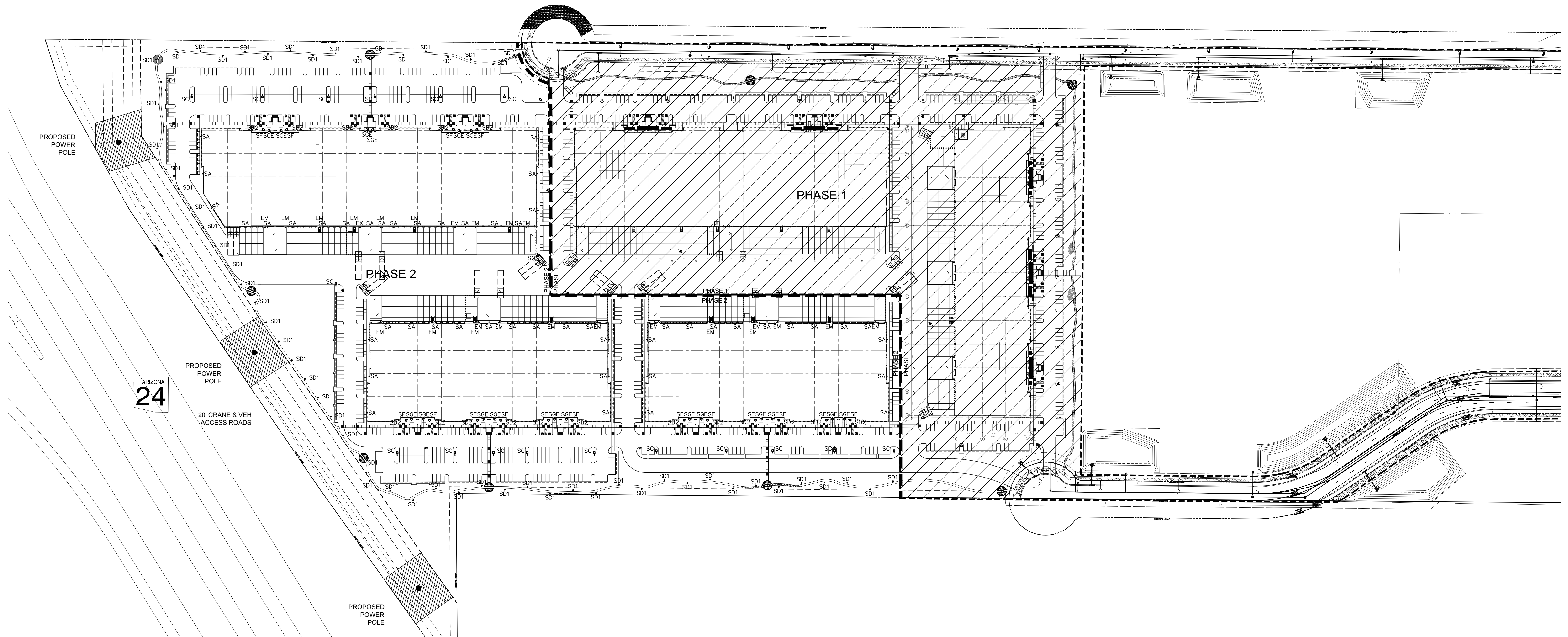
SITE LIGHTING PLAN
