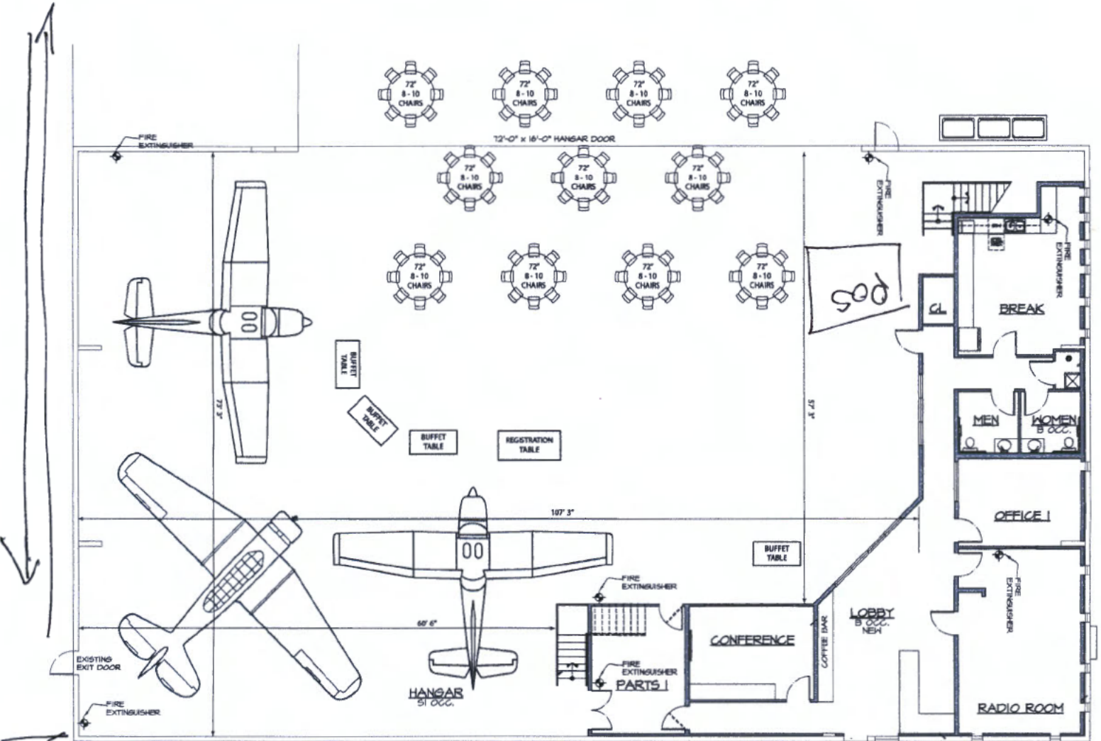
FLOOR PLAN "EVFFC"
