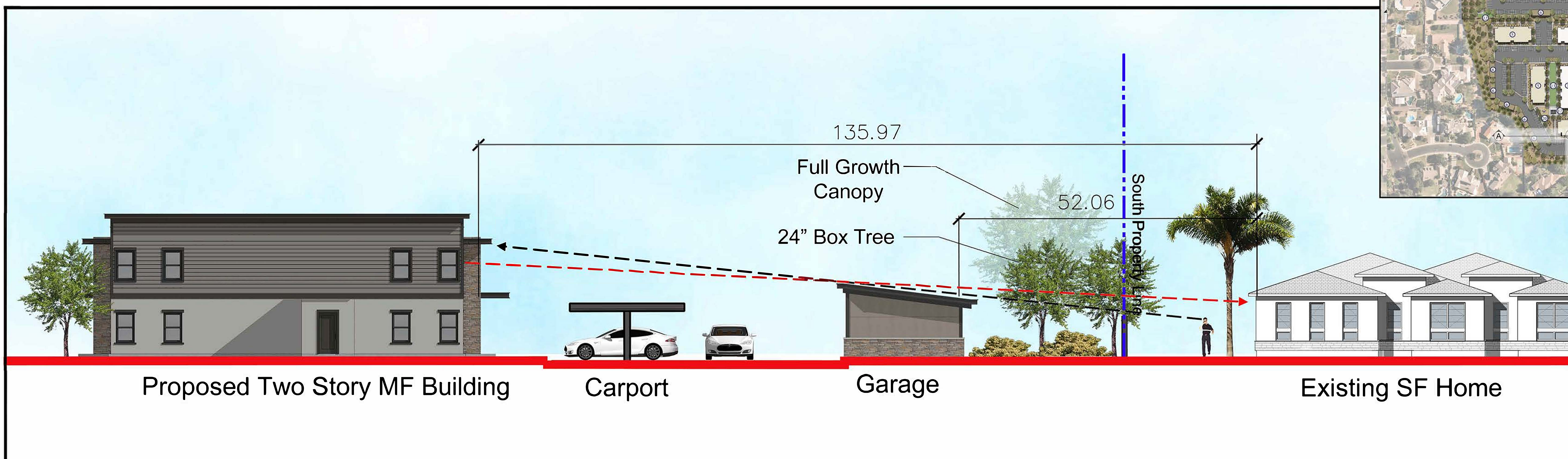
SECTION B
