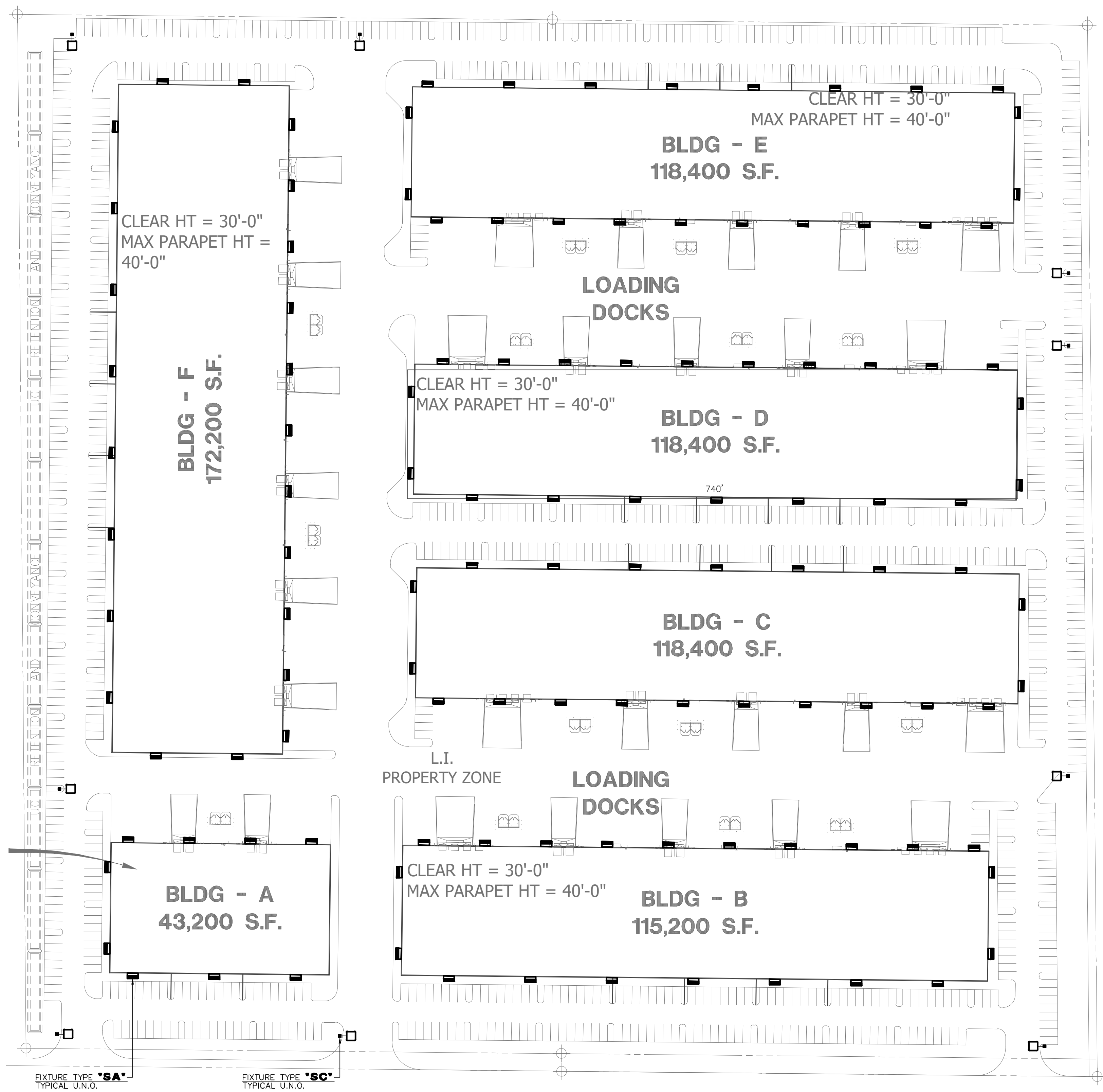
SITE LIGHTING PLAN SCALE: 1" = 80'-0"
