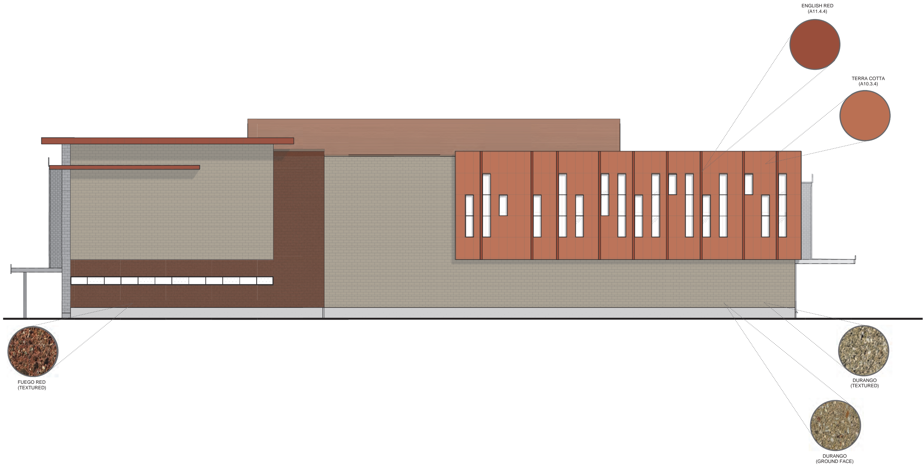
EXTERIOR ELEVATION - NORTH
