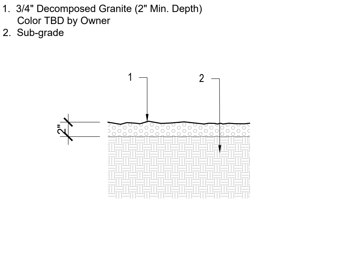
14 D.G. TOP DRESS DETAIL SCALE: NTS
