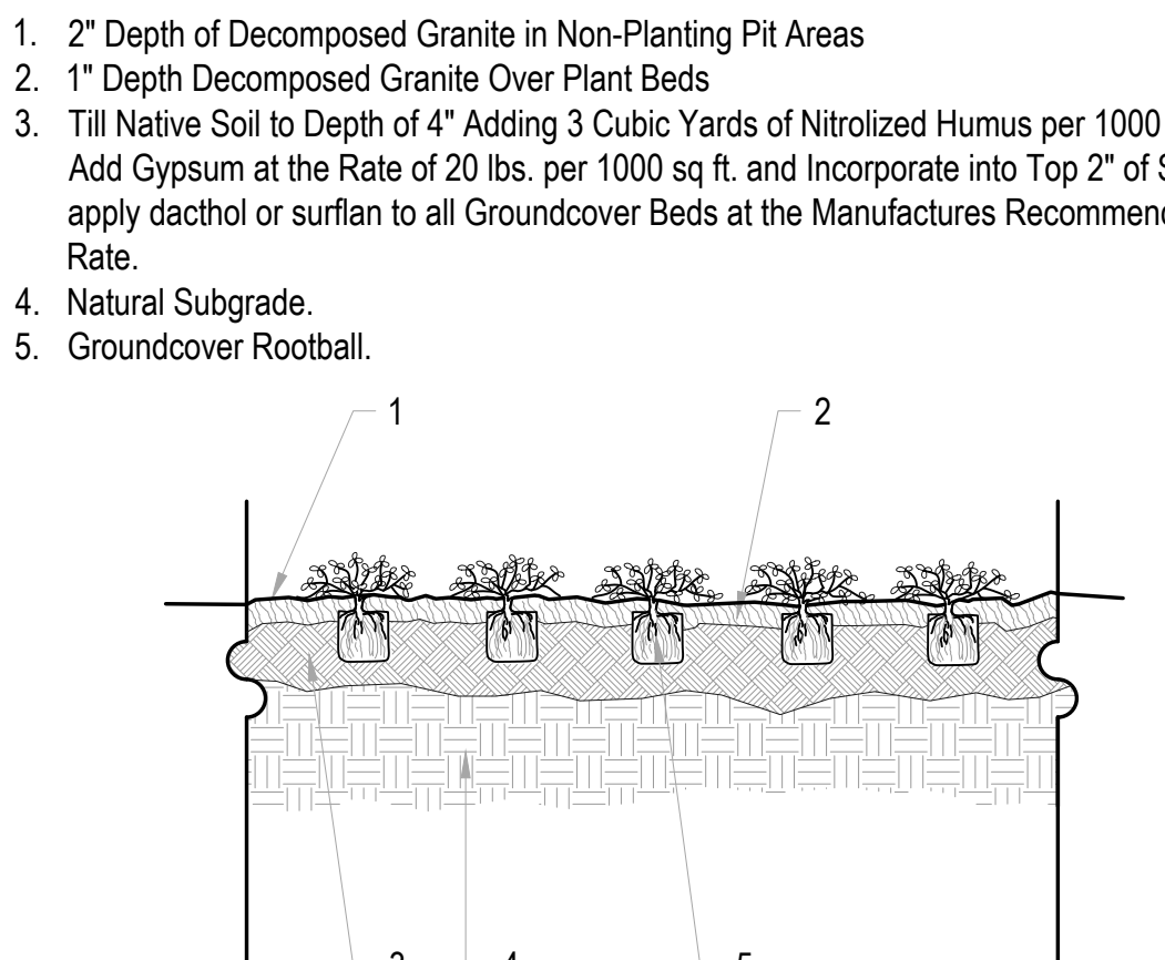
12 GROUND COVER PLANTING SCALE: NTS
