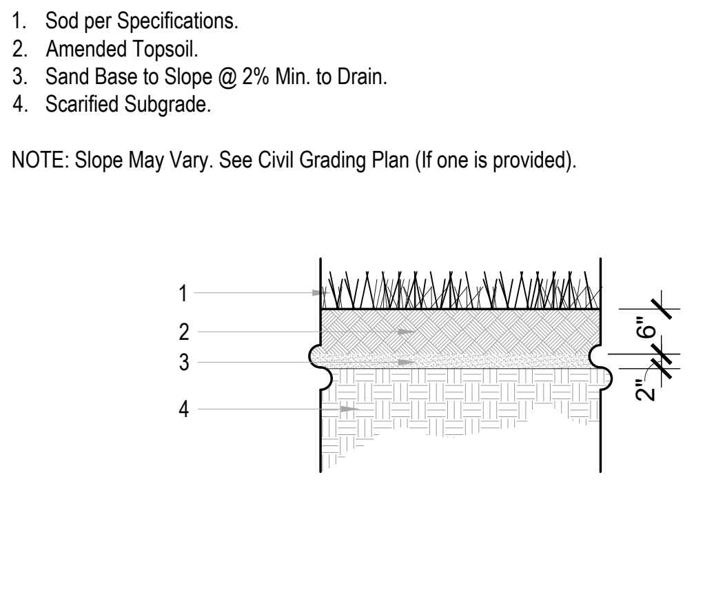
10 TURF PLANTING DETAIL SCALE: NTS
