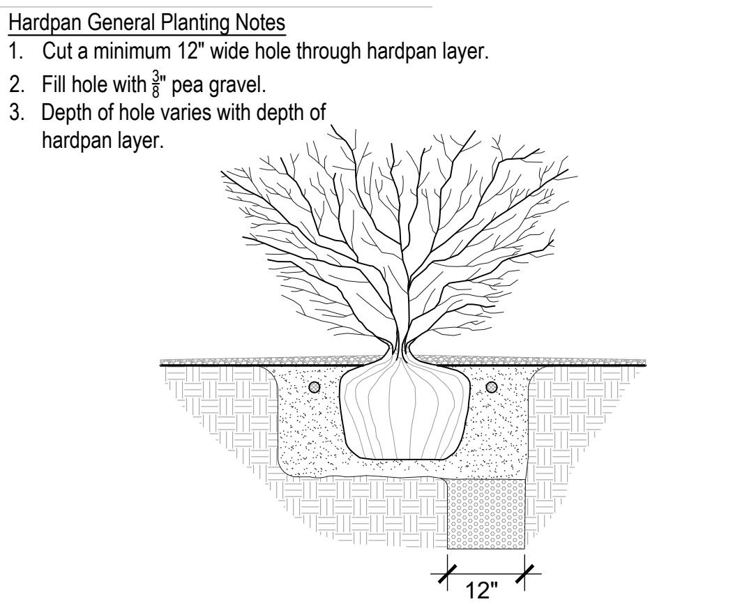
17 PLANTING IN HARDPAN DETAIL SCALE: NTS
