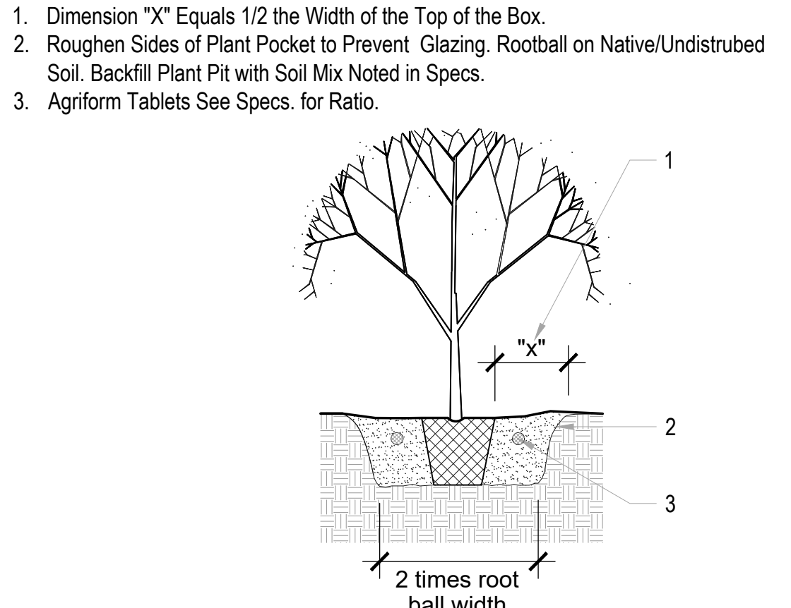
2 24" BOX TREE & LARGER SCALE: NTS
