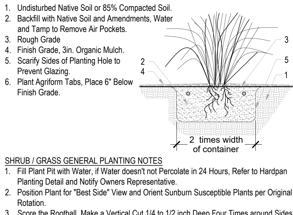
6 GRASS PLANTING DETAIL SCALE: NTS
