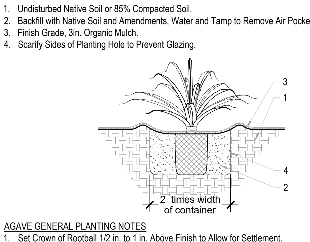
7 AGAVE PLANTING DETAIL SCALE: NTS
