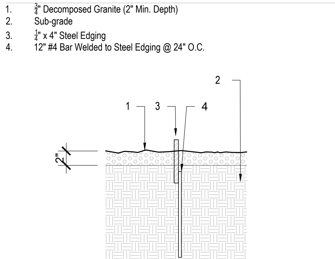
16 STEEL EDGING DETAIL SCALE: NTS
