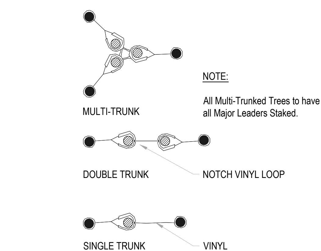
5 TREE GUYING DETAIL SCALE: NTS
