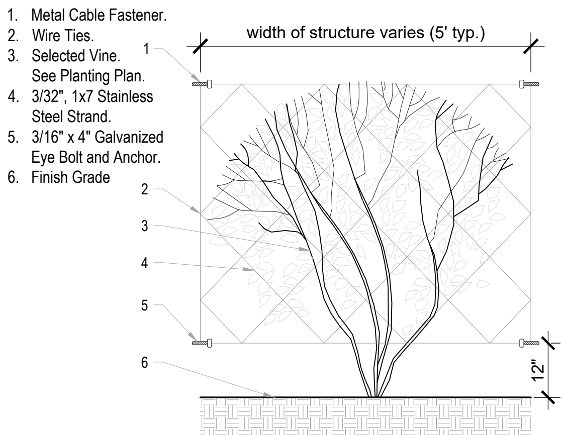
13 VINE ON TRELLIS DETAIL SCALE: NTS
