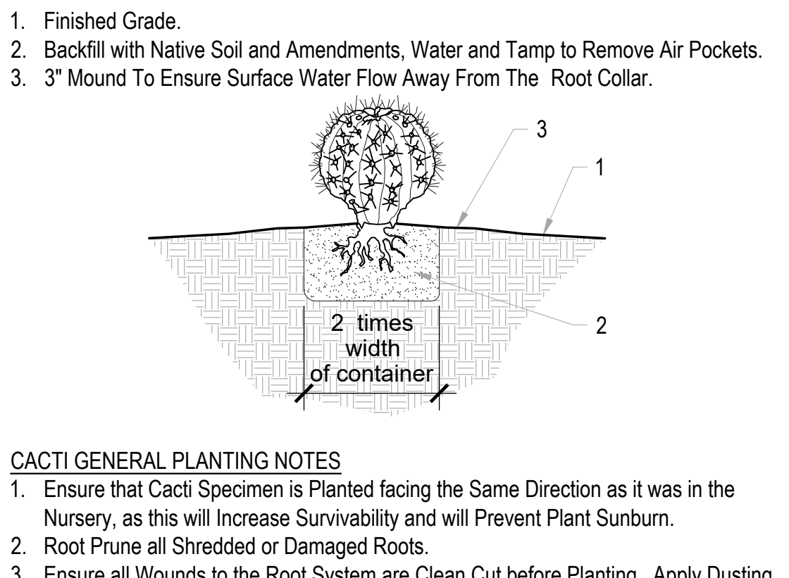
8 CACTI PLANTING DETAIL SCALE: NTS
