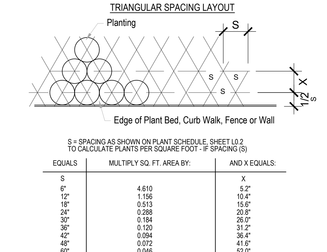
11 PLANT SPACING SCALE: NTS
