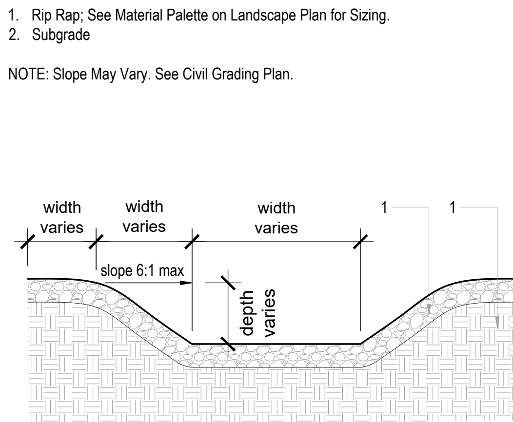
15 SWALE DETAIL SCALE: NTS
