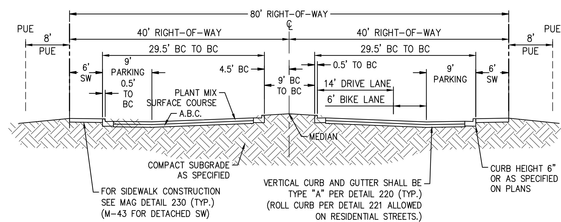
5 LOCAL COLLECTOR STREET SECTION (WITH PARKING) PRATT AVE, PRAIRIE AVE & PRIMROSE N.T.S.
