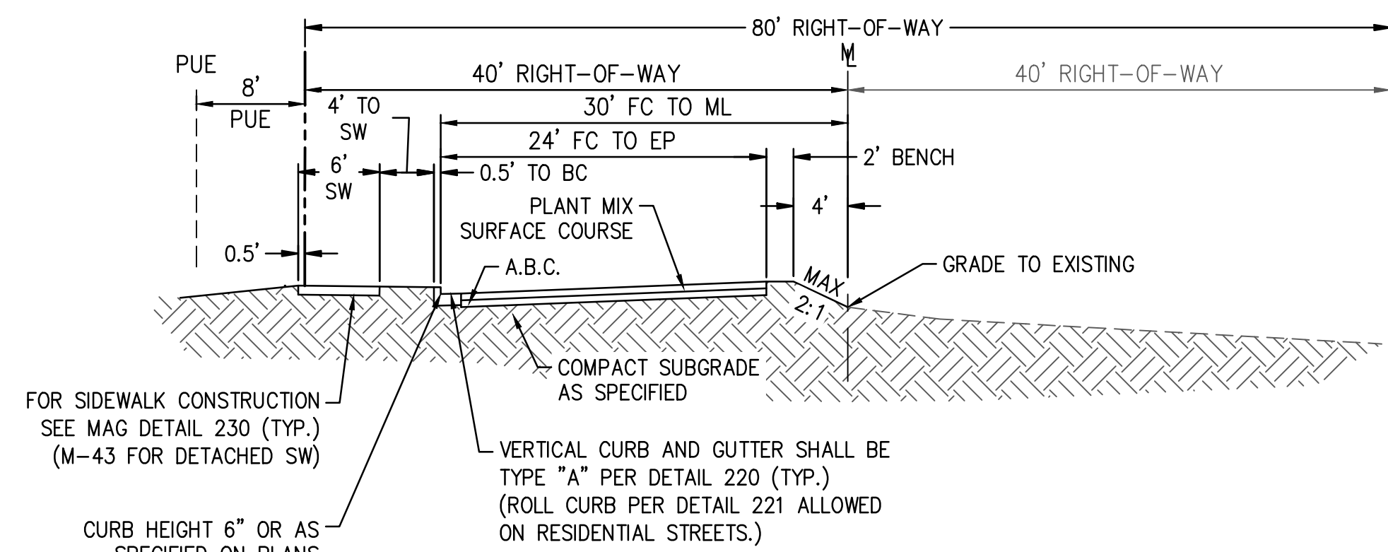
10 COLLECTOR STREET SECTION (INTERIM HALF-STREET) 82ND STREET LOOKING NORTH N.T.S.
