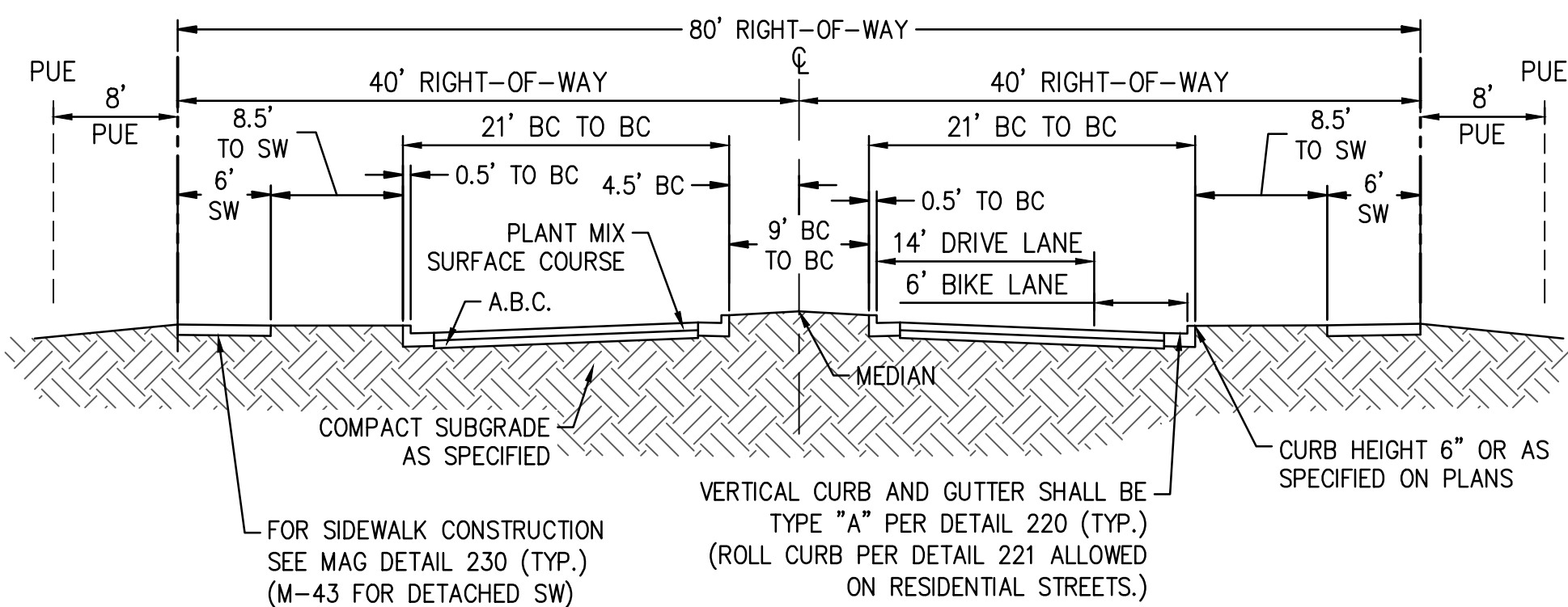
2 LOCAL COLLECTOR STREET SECTION (WITHOUT PARKING) PRATT AVE, PRAIRIE AVE & PRIMROSE N.T.S.
