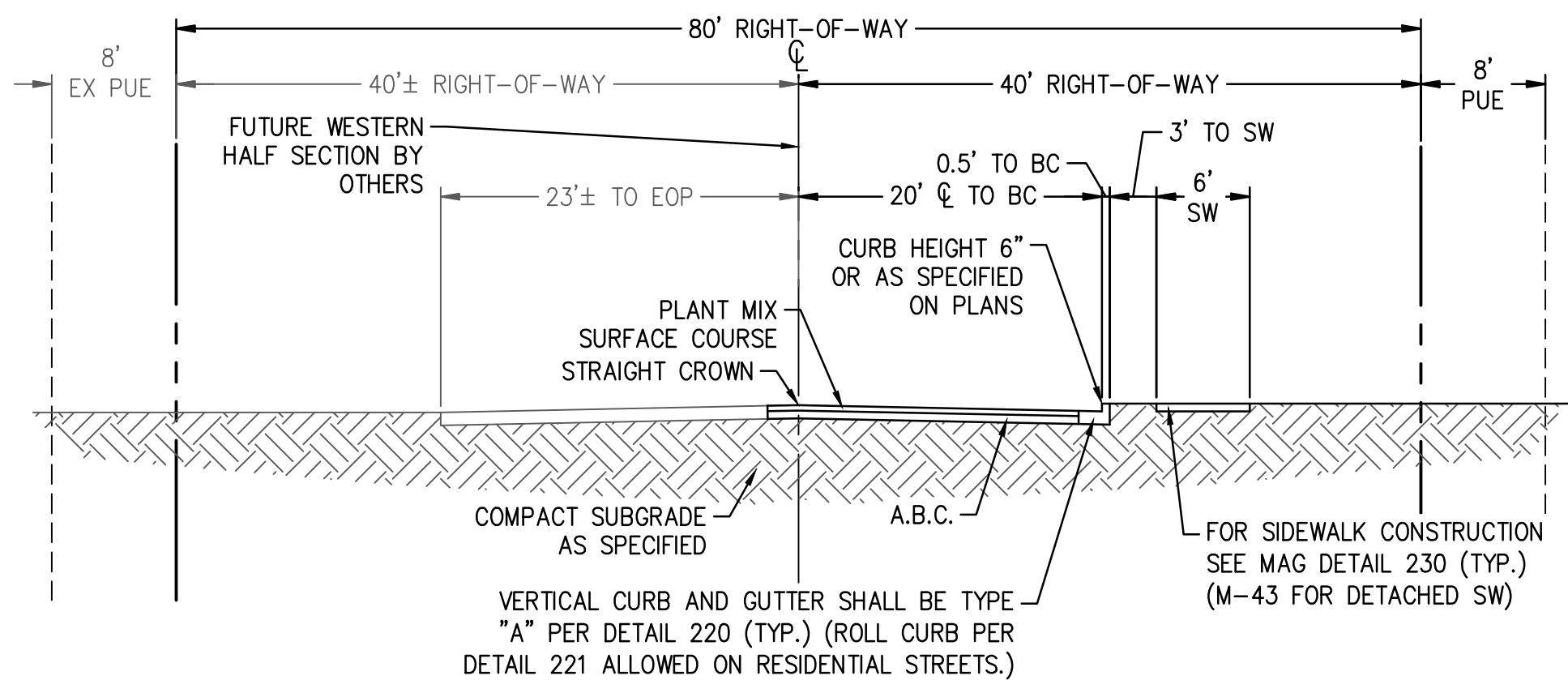
4 COLLECTOR STREET SECTION (EASTERN HALF-STREET) 80TH STREET LOOKING NORTH N.T.S.
