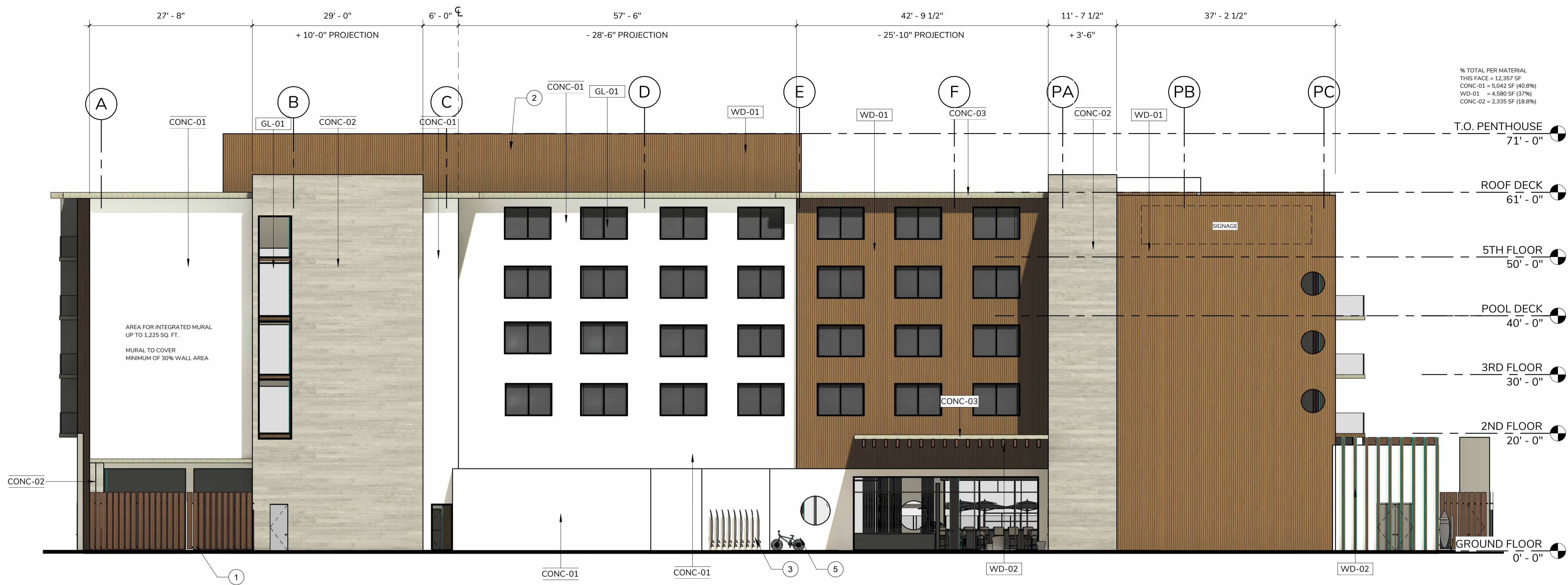
1 WEST ELEVATION 3/32" = 1'-0"
