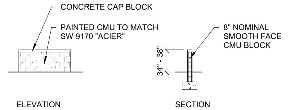
3 SCREEN WALL 1/8" = 1'-0"
