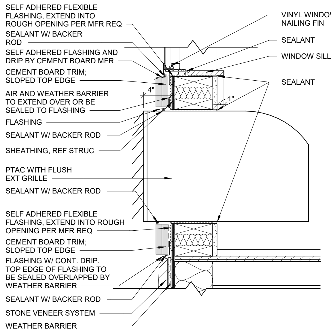
7 WINDOW SILL - STONE 1 1/2" = 1'-0" REF: A610 / A
