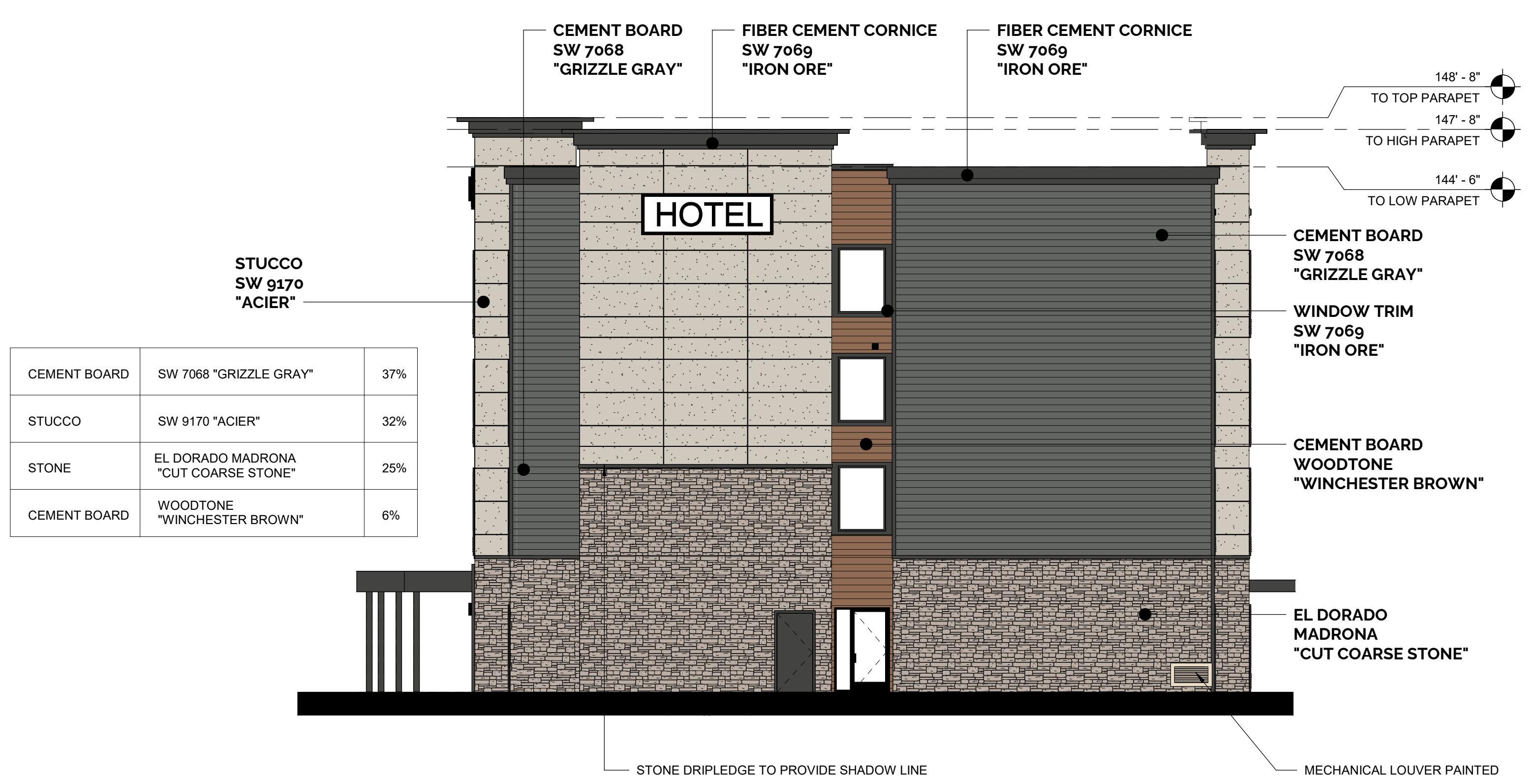
1 WEST (LEFT) ELEVATION 1/8" = 1'-0" REF: SD1.1 / 1
