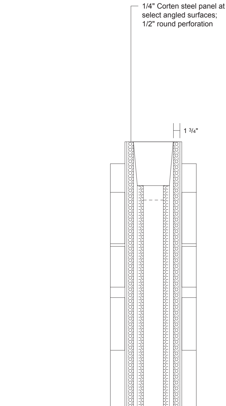
W-3.01 Monument ID (Side) Scale: 3/4\" = 1'-0"
