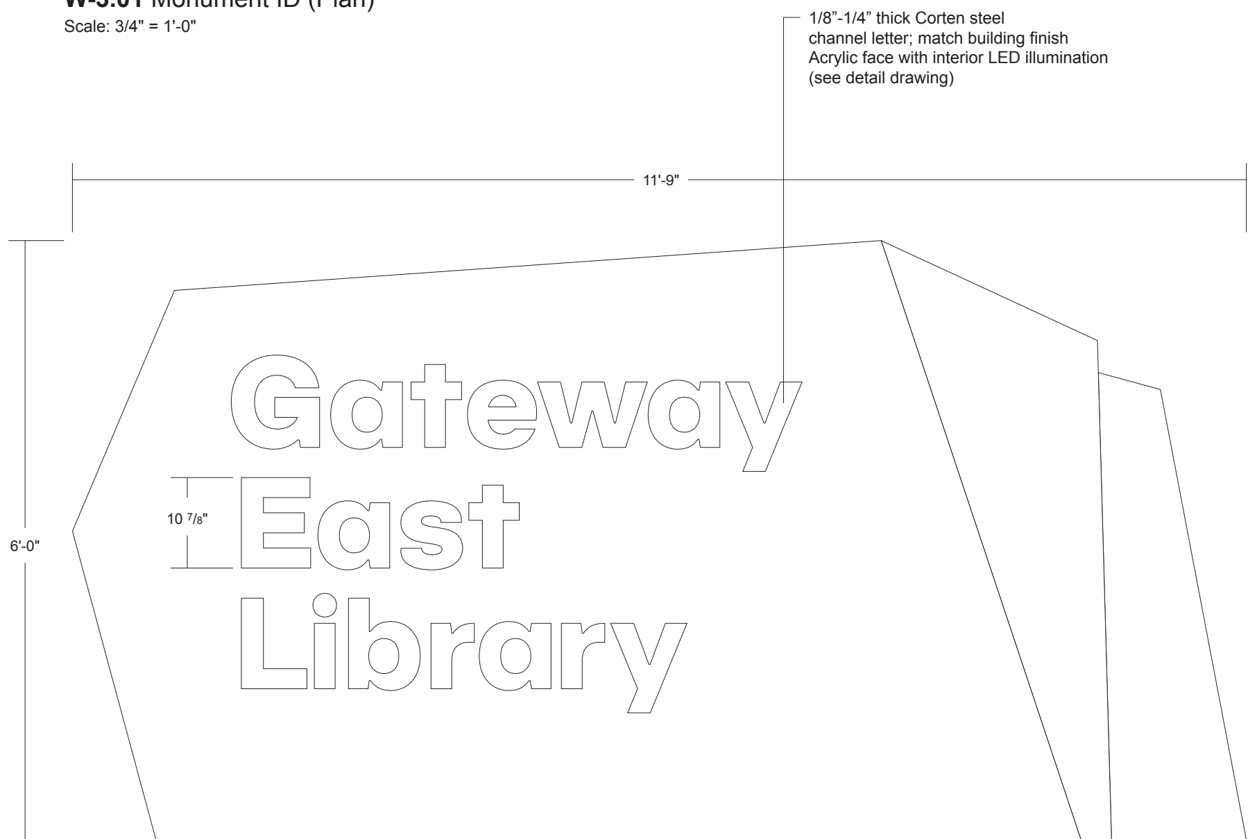
W-3.01 Monument ID - Front Scale: 3/4\" = 1'-0"
