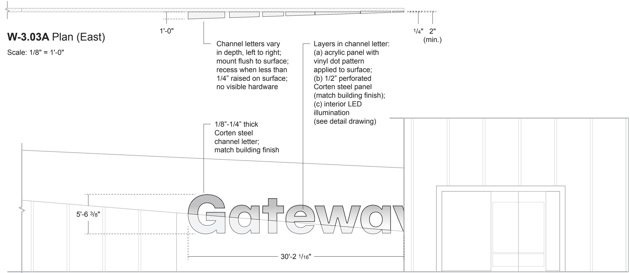
W-3.03A Elevation (East) Scale: 1/8\" = 1'-0"
