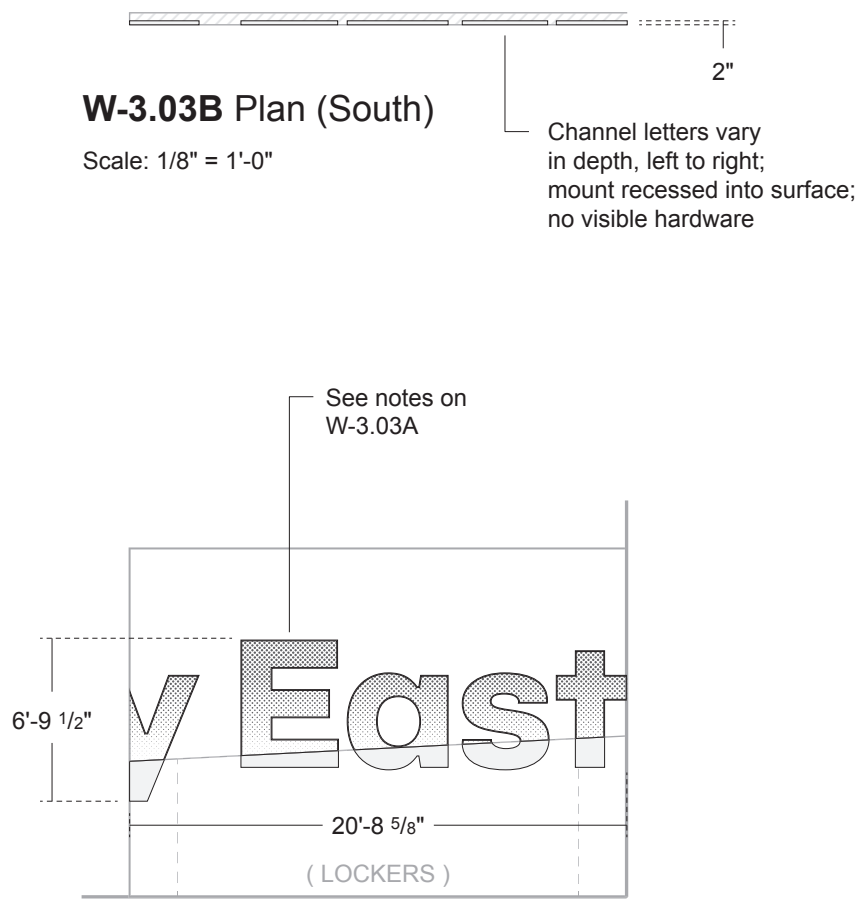
W-3.03B Elevation (South) Scale: 1/8\" = 1'-0"
