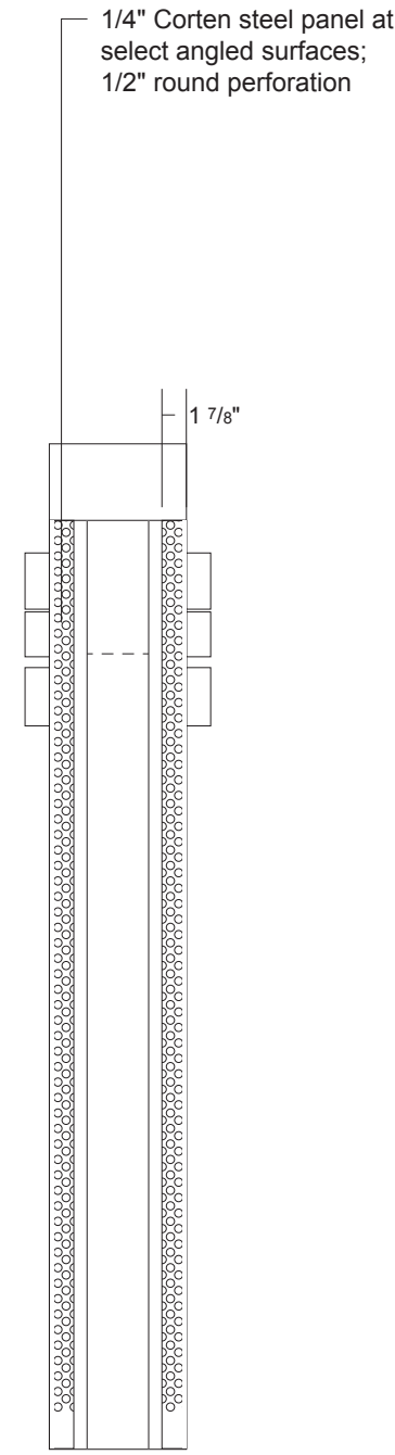
W-3.02 Auxiliary Monument ID (Side) Scale: 3/4\" = 1'-0"
