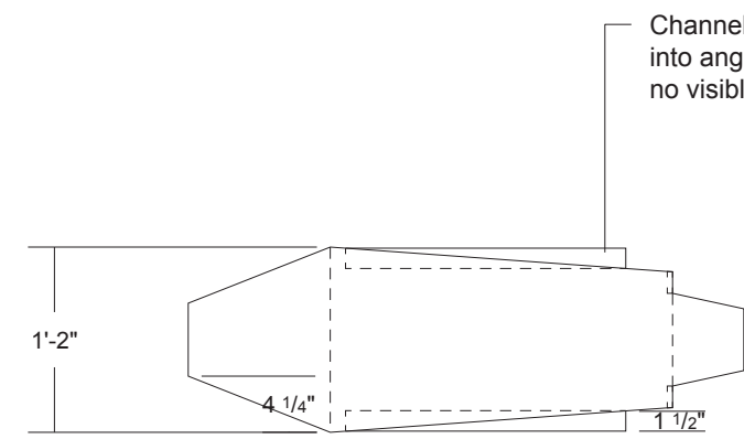
W-3.02 Auxiliary Monument ID (Plan) Scale: 3/4\" = 1'-0"
