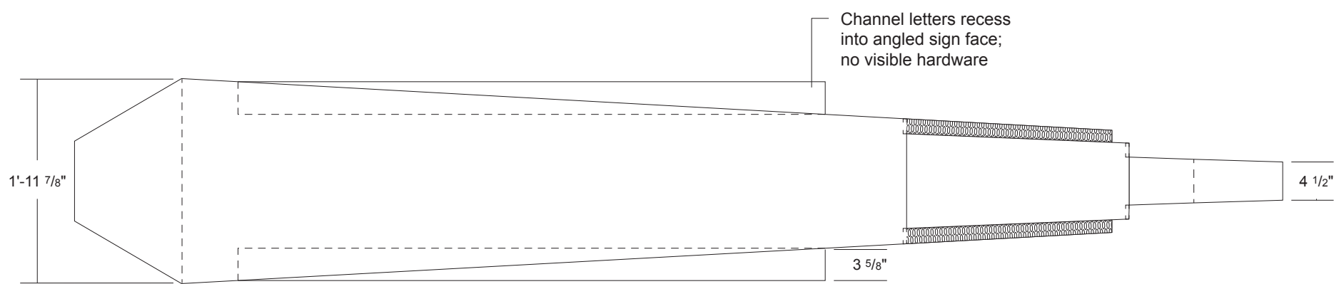
W-3.01 Monument ID (Plan) Scale: 3/4\" = 1'-0"
