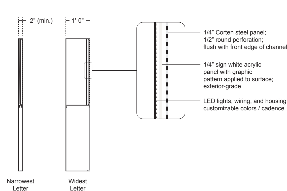
W-3.03 Detail (Channel Letter) Scale: 1/2\" = 1'-0"
