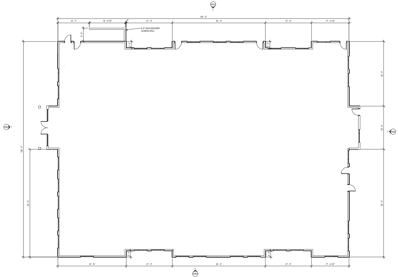
1 PROPOSED FLOOR PLAN 1/8" = 1'-0"
