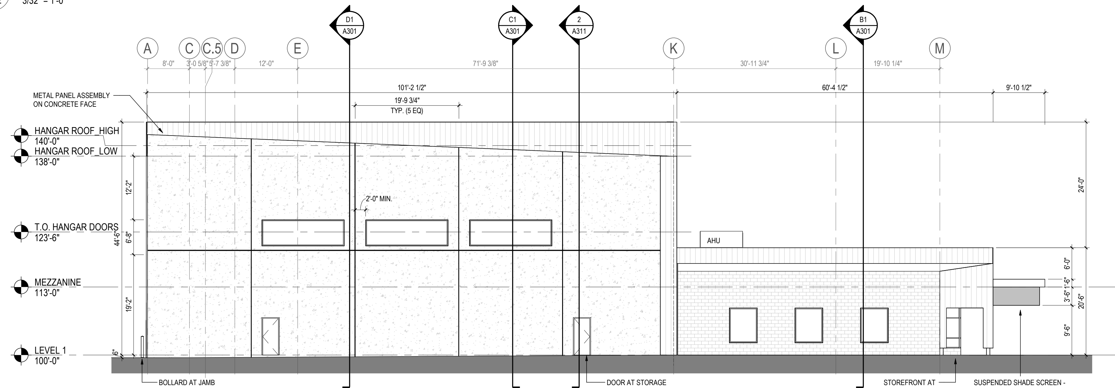
C1 WEST ELEVATION A202 3/32" = 1'-0"
