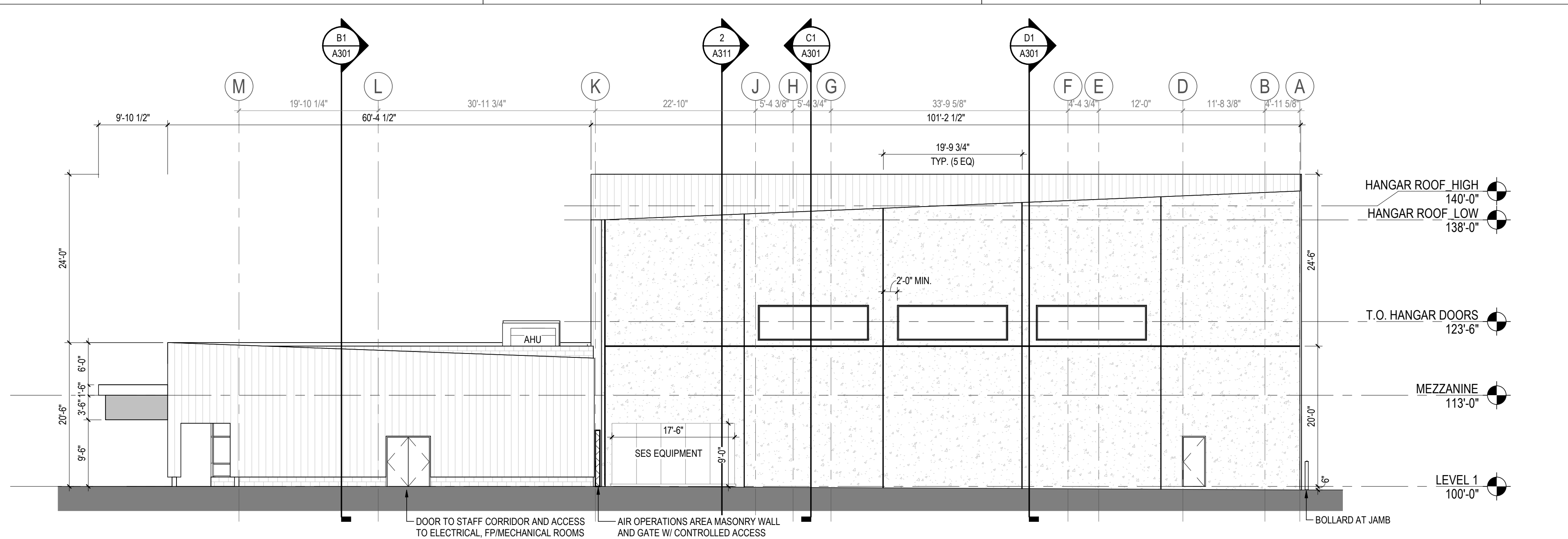
D1 EAST ELEVATION A202 3/32" = 1'-0"
