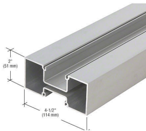
ALUMINUM STOREFRONT MANUFACT: KAWNEER COLOR: CLEAR ANODIZED
