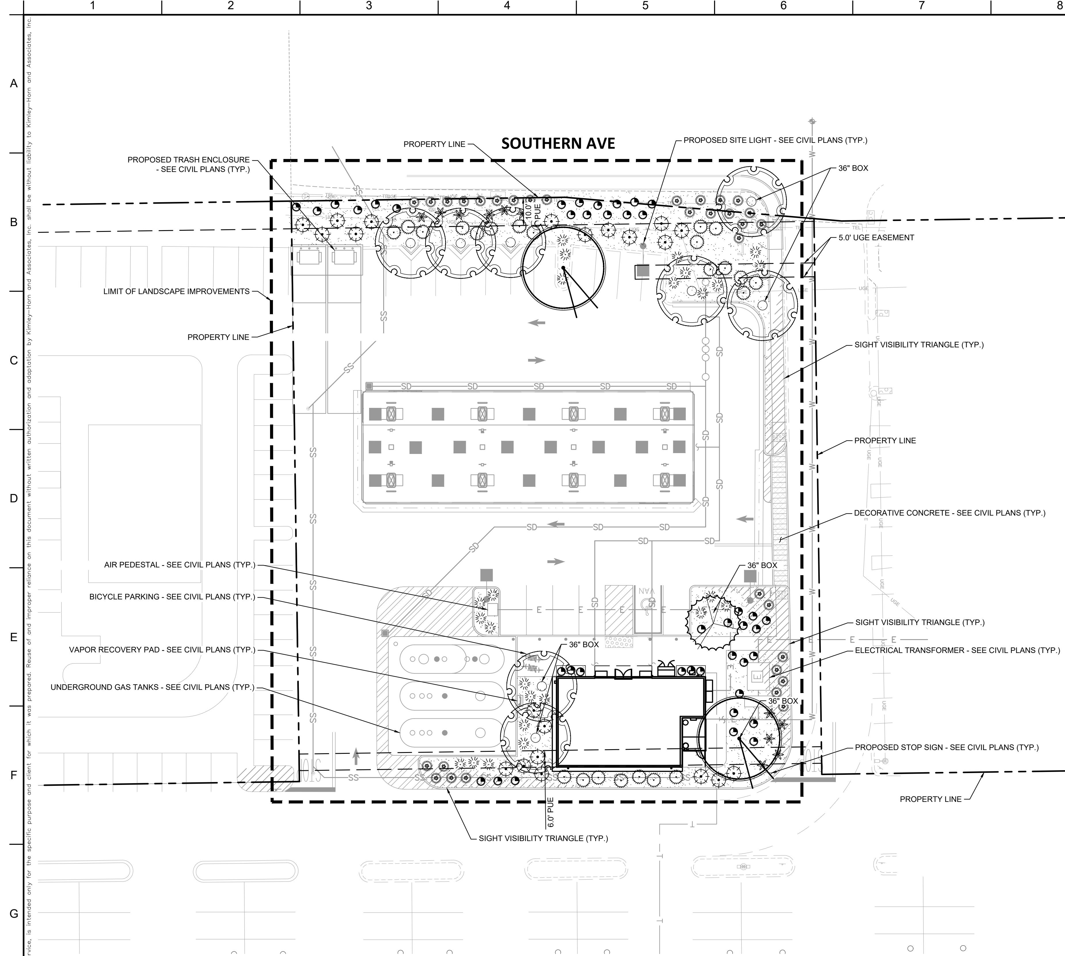
A FINAL LANDSCAPE PLAN 1" = 20"
