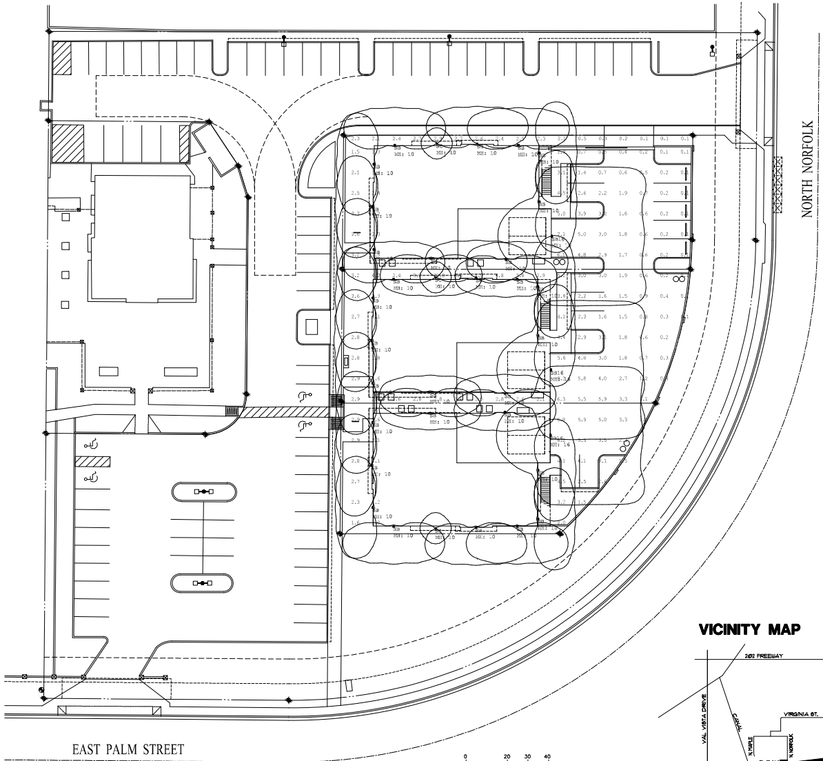
PHOTOMETRIC PLAN
