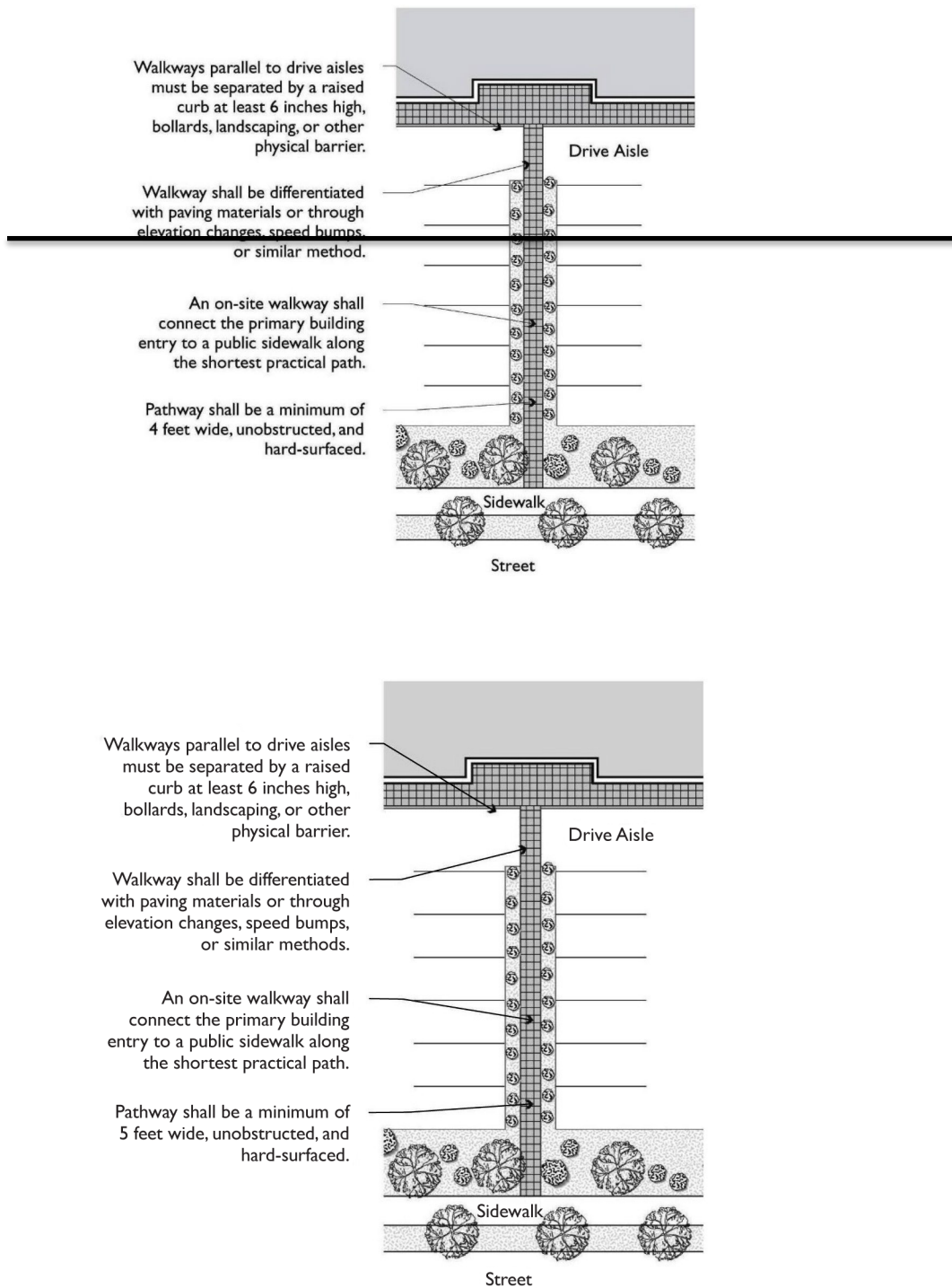
FIGURE 11-30-8.A(1): PEDESTRIAN ACCESS THROUGH PARKING AREA
