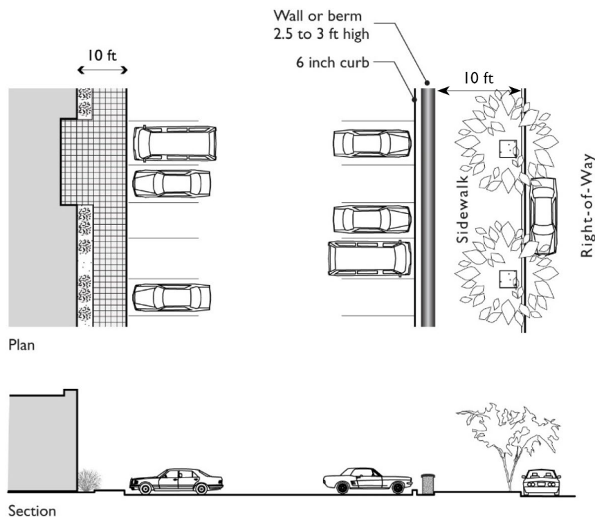
FIGURE 11-30-9.G(1): SCREENING AND SEPARATION OF PARKING AREA
