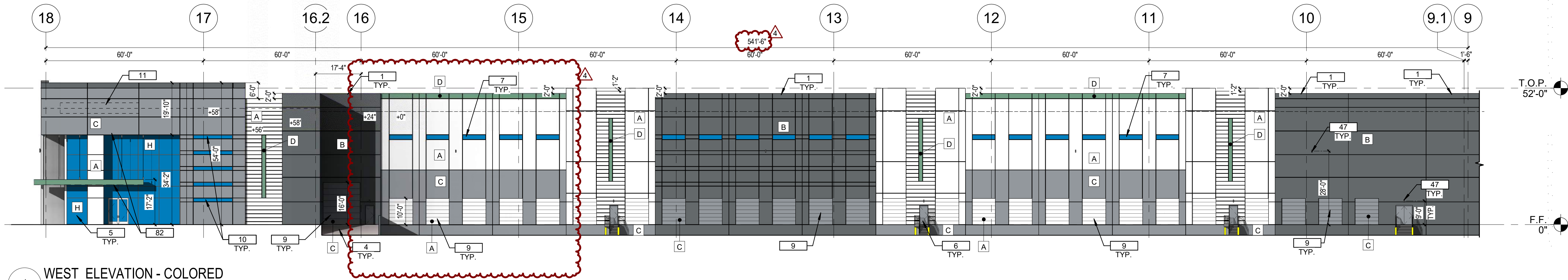
1 WEST ELEVATION - COLORED SCALE 0' 16' 32' 64' 80' 3/64" = 1'-0"
