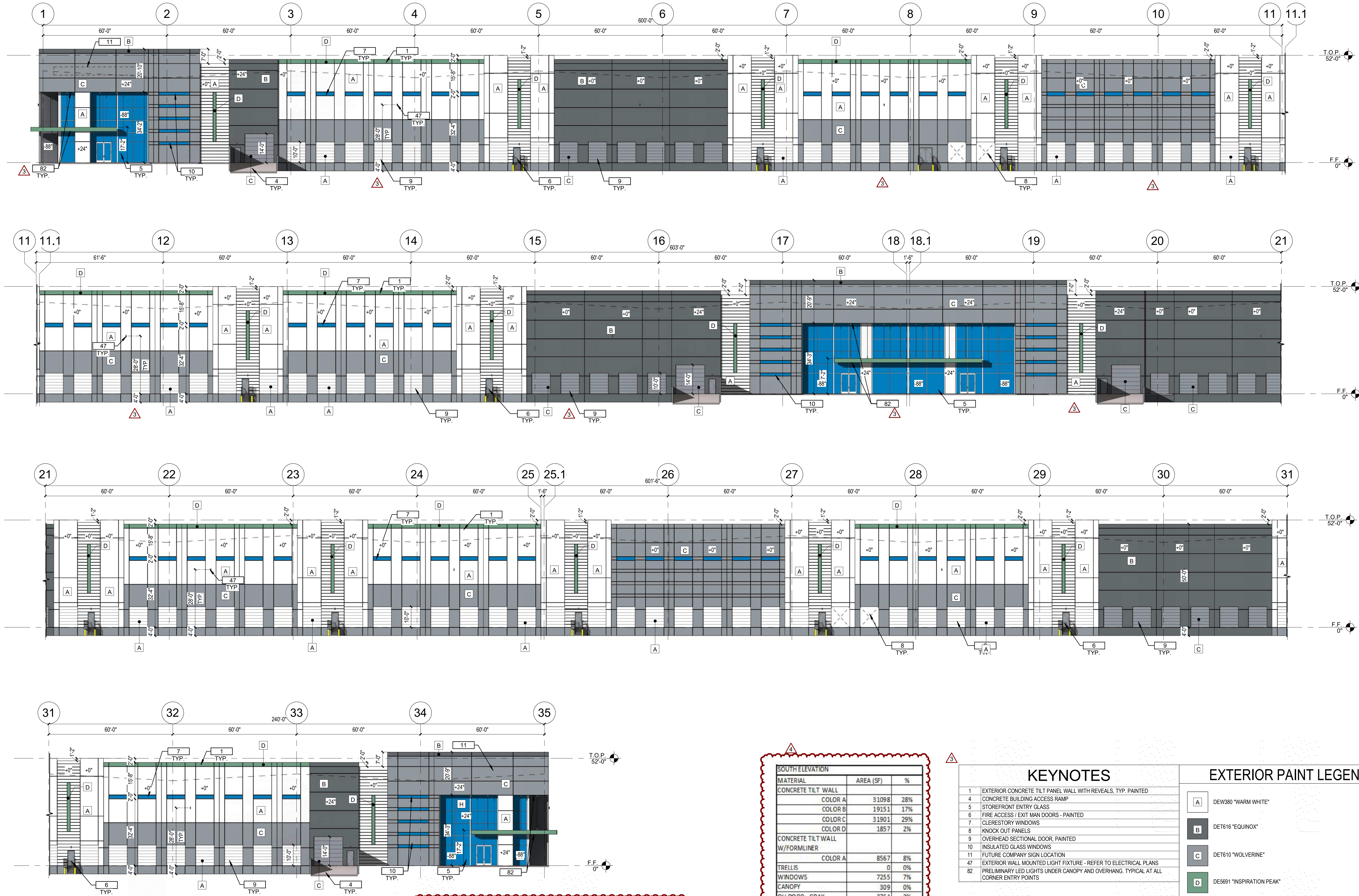
1 SOUTH ELEVATION - COLORED
