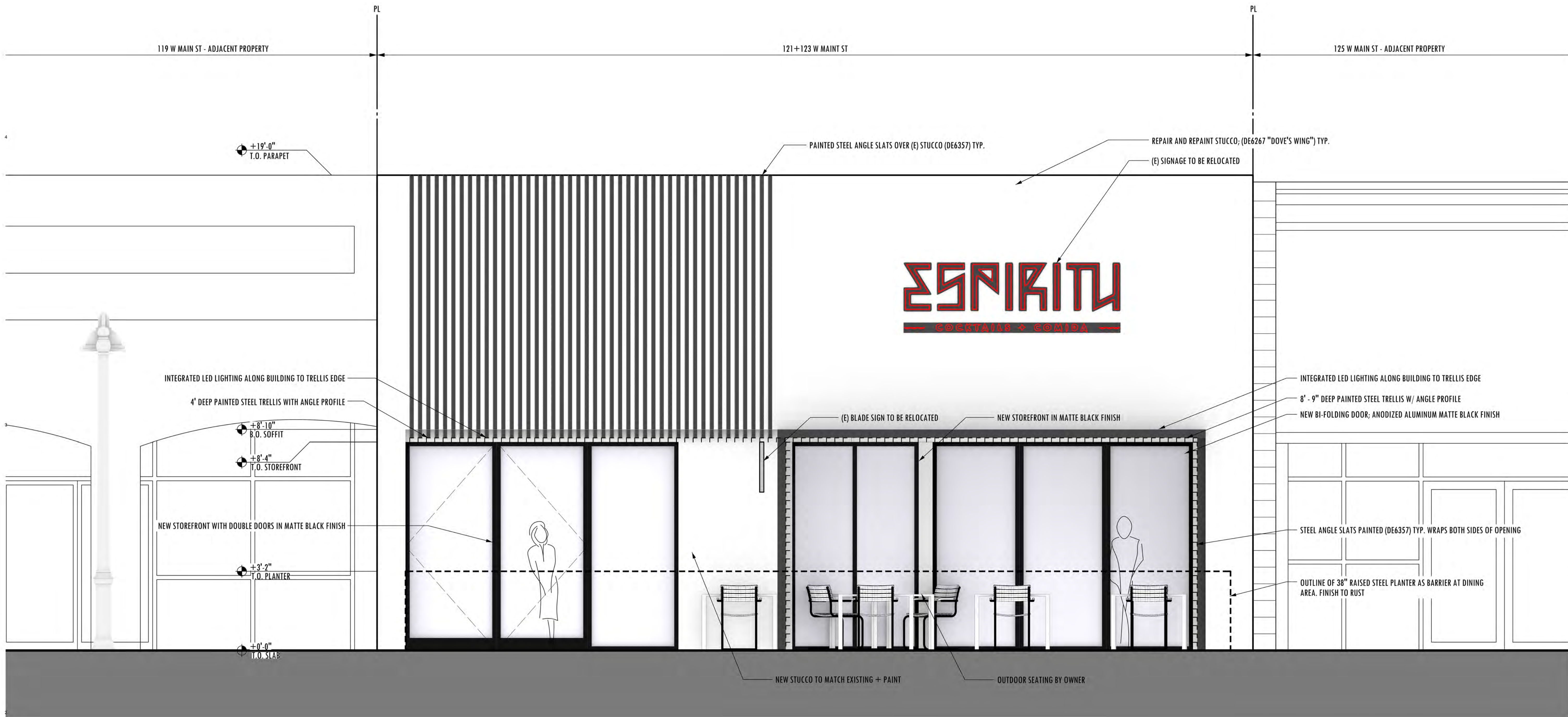
1 S MAIN ST ELEVATION 1/2" = 1'-0" 0 1' 2' 5' 10'
