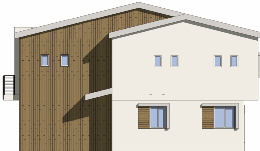
3 SIDE END ELEVATION 1/4" = 1'-0"
