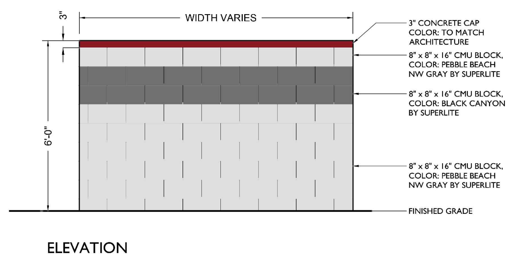
4 6' TRASH ENCLOSURE WALL & PERIMETER WALL Scale: 1/2" = 1'-0"
