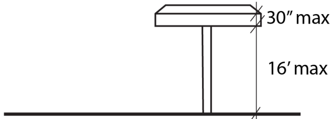
FIGURE 11-31-25.C: PUMP FUELING CANOPY DIMENSIONS
