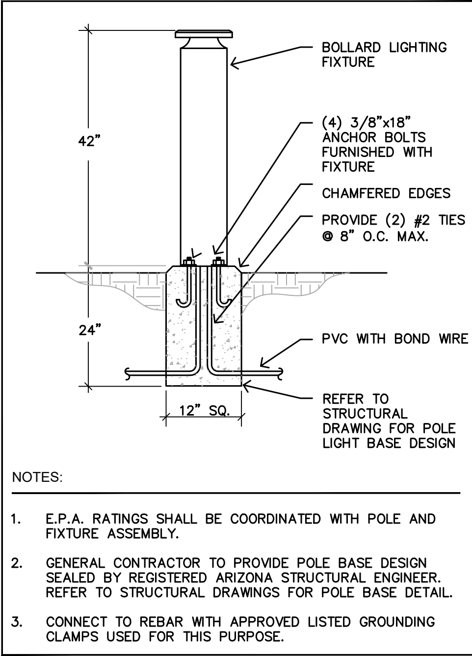
3 BOLLARD LIGHTING DETAIL 'BO' SCALE : NONE
