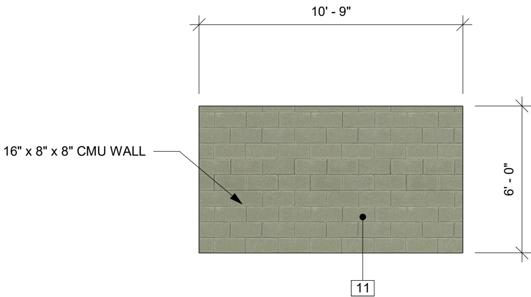
LEFT ELEVATION
