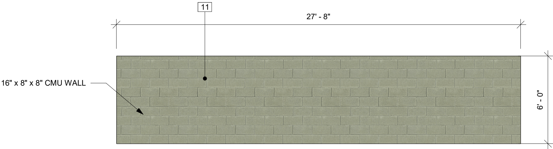
BACK ELEVATION
