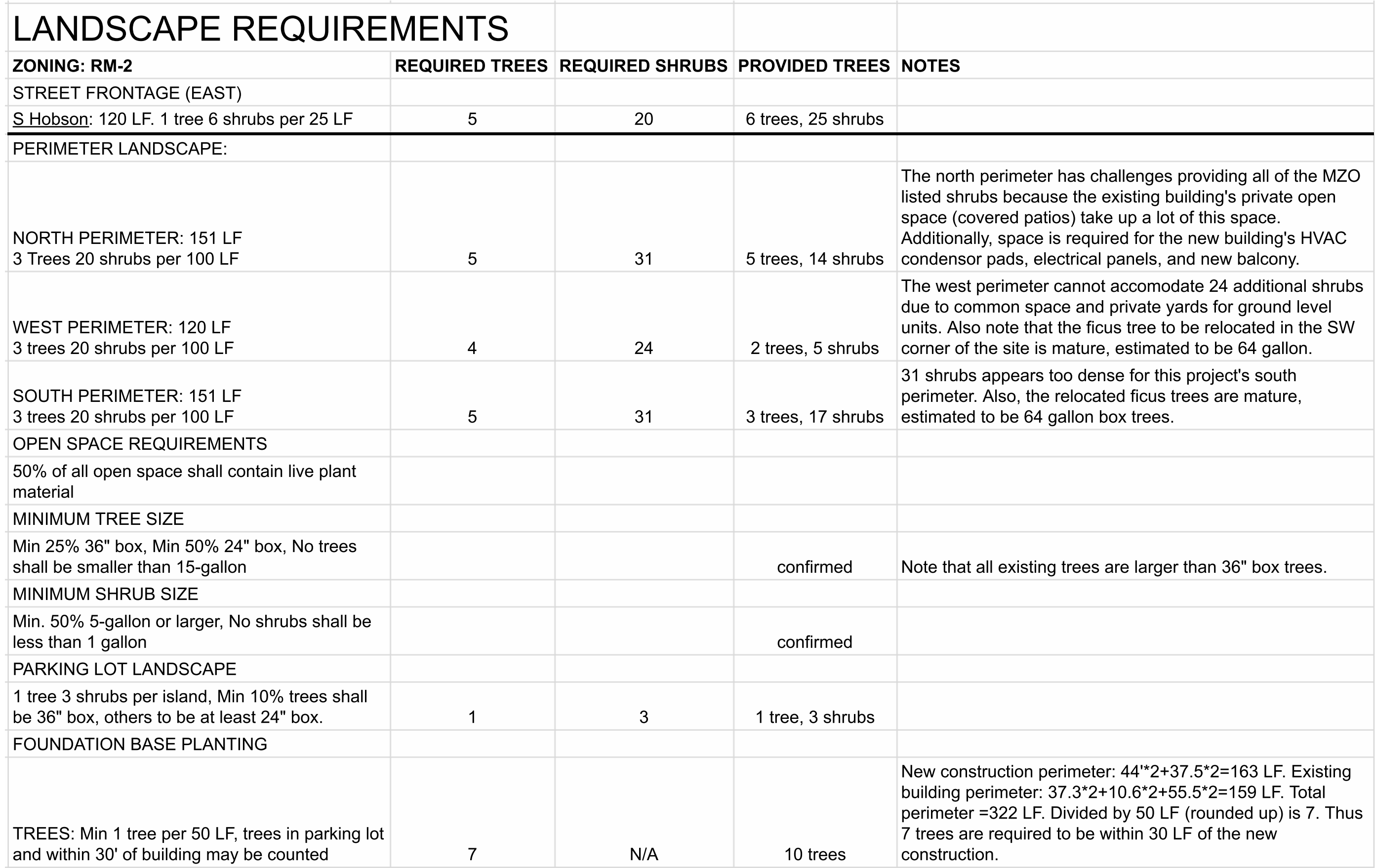
LANDSCAPE PLAN 1/8" = 1 FT
