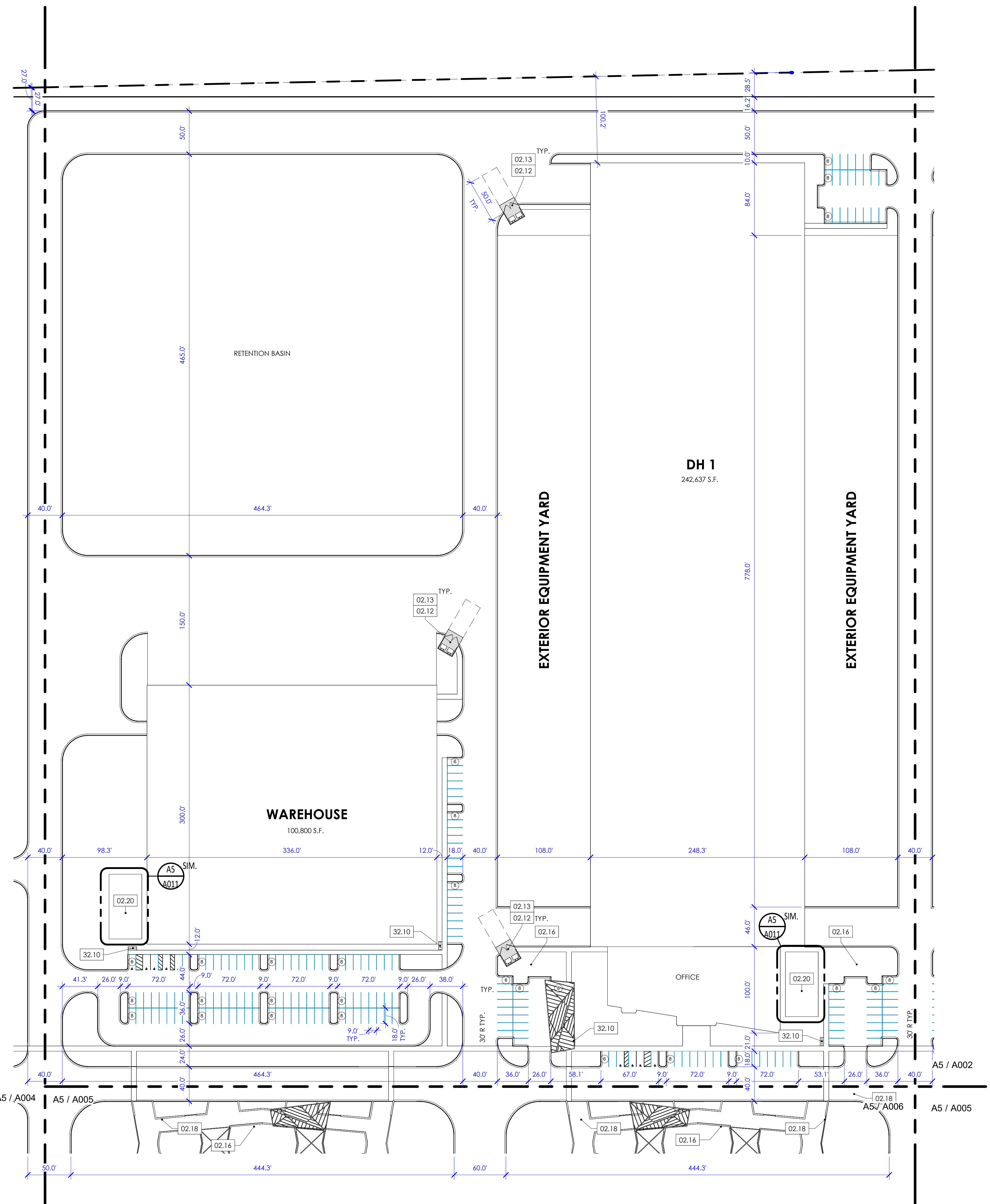
A5 A003 SITE PLAN - ENLARGED AREA B 1" = 60'-0"
