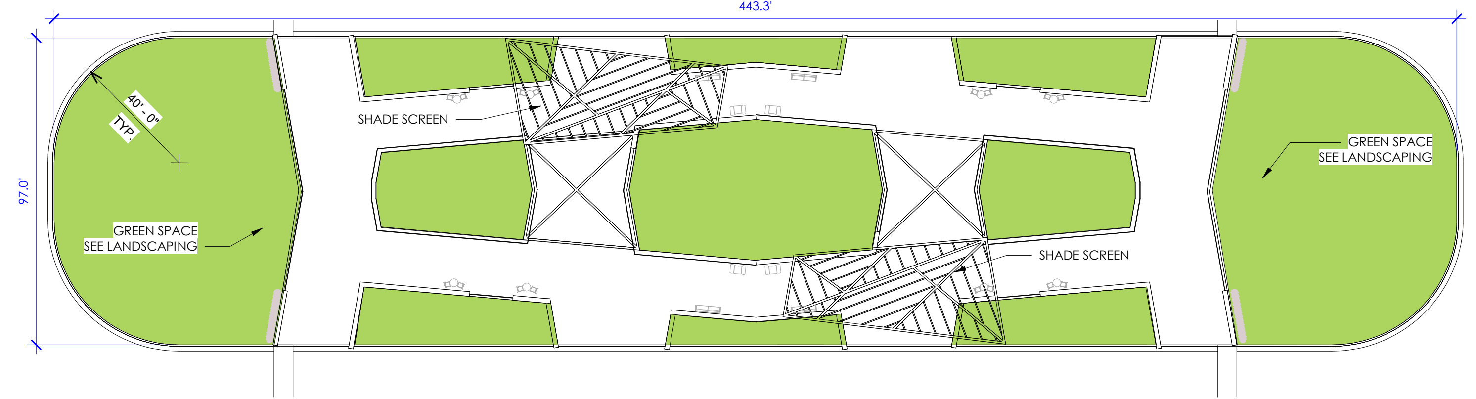
D2 ENLARGED CENTRAL AMENITY SPACE 1" = 30'-0"
