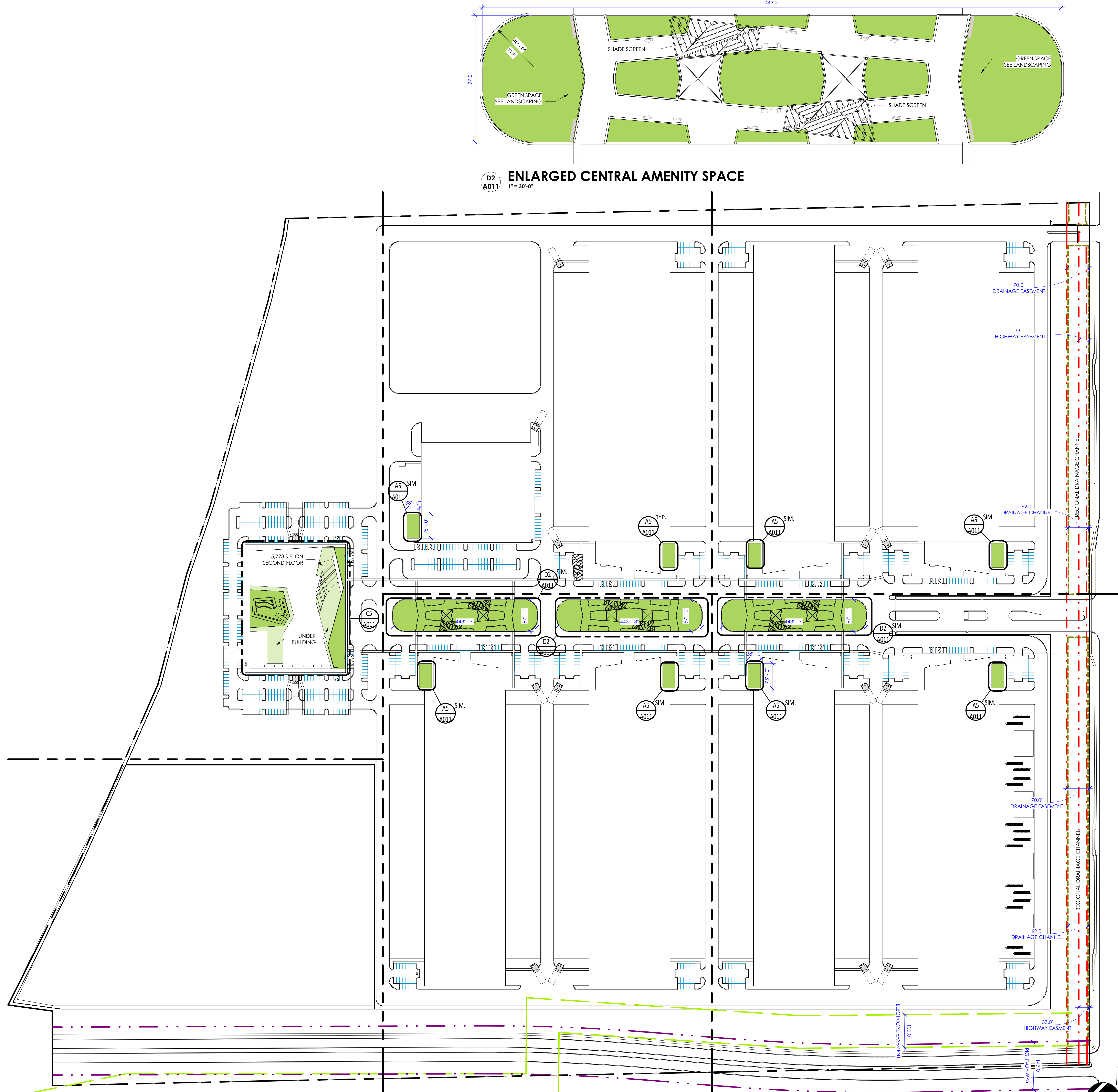
A4 SITE AMENITY PLAN 1" = 120'-0"
