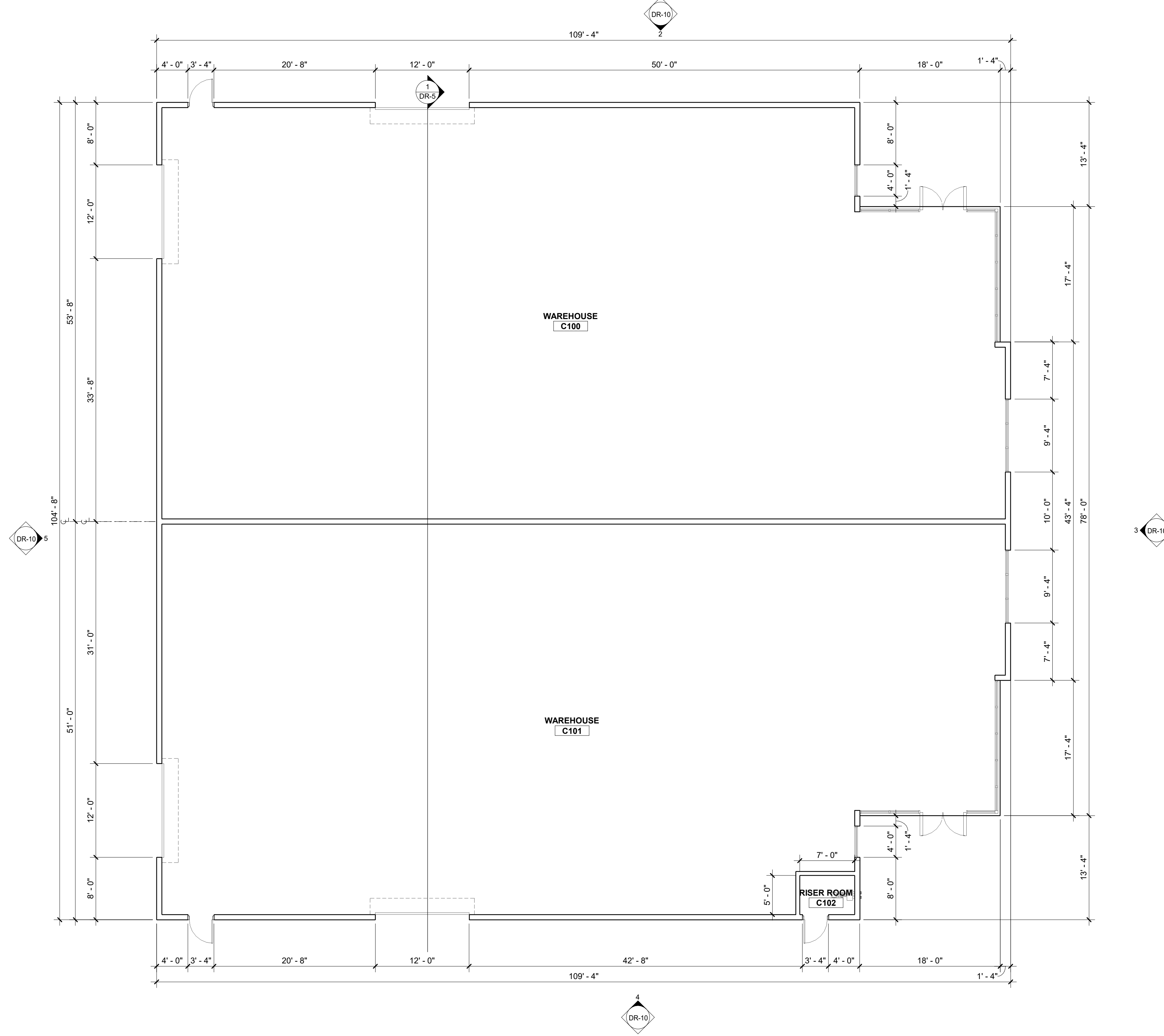
BUILDING C FLOOR PLAN
