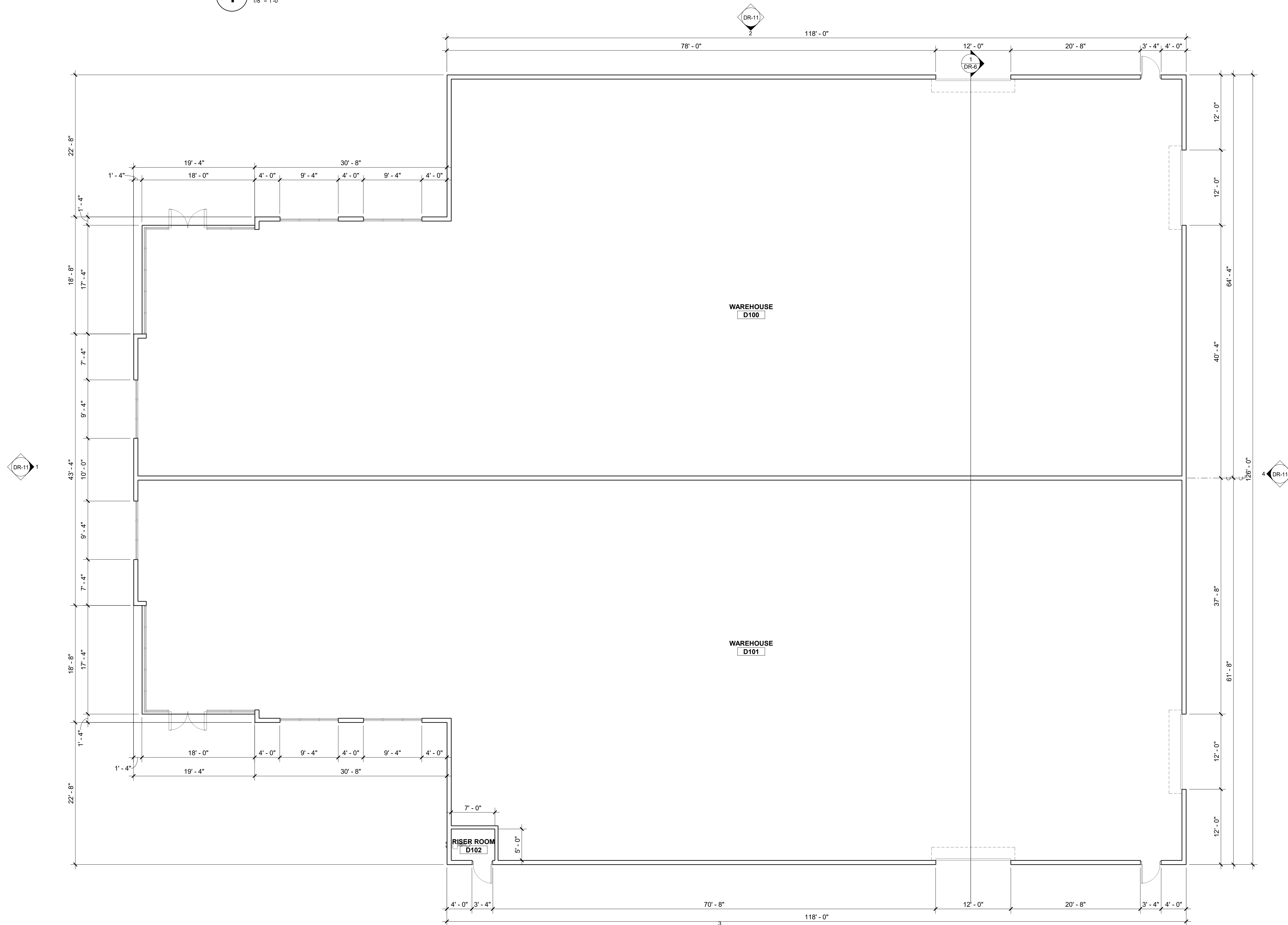
BUILDING D FLOOR PLAN 1/8" = 1'-0"
