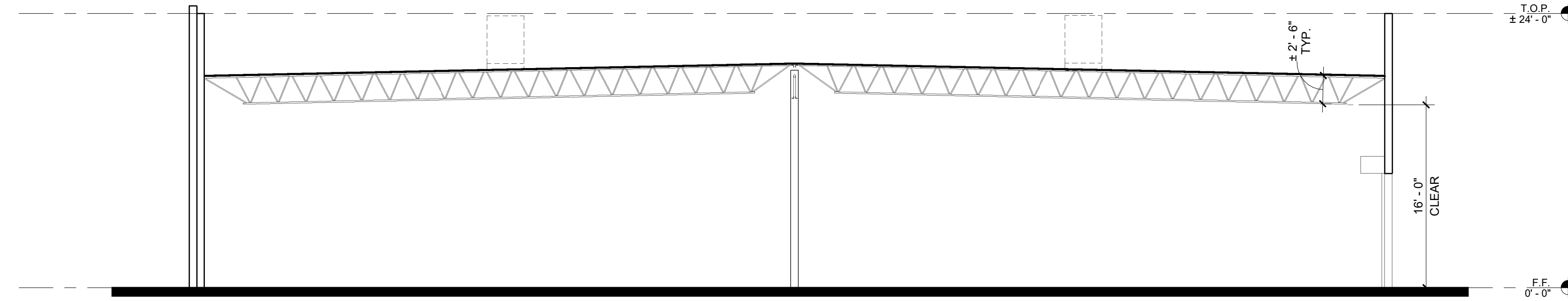
1 BUILDING A SECTION 1/8" = 1'-0"
