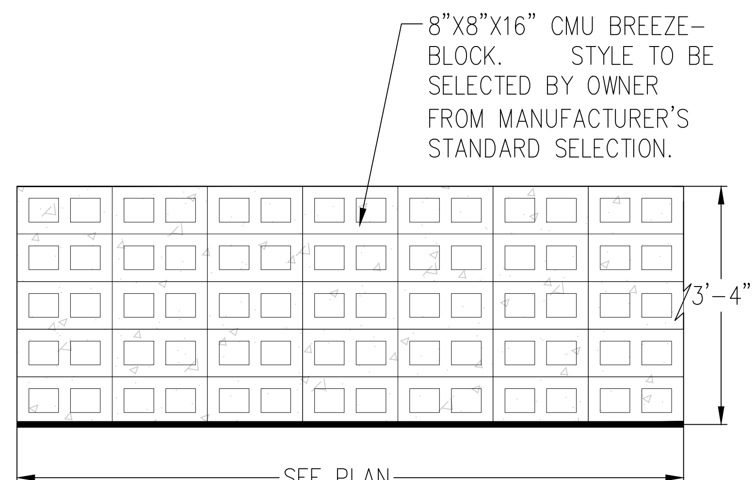
4 40" DECORATIVE WALL SCALE: 3/4" = 1'-0"
