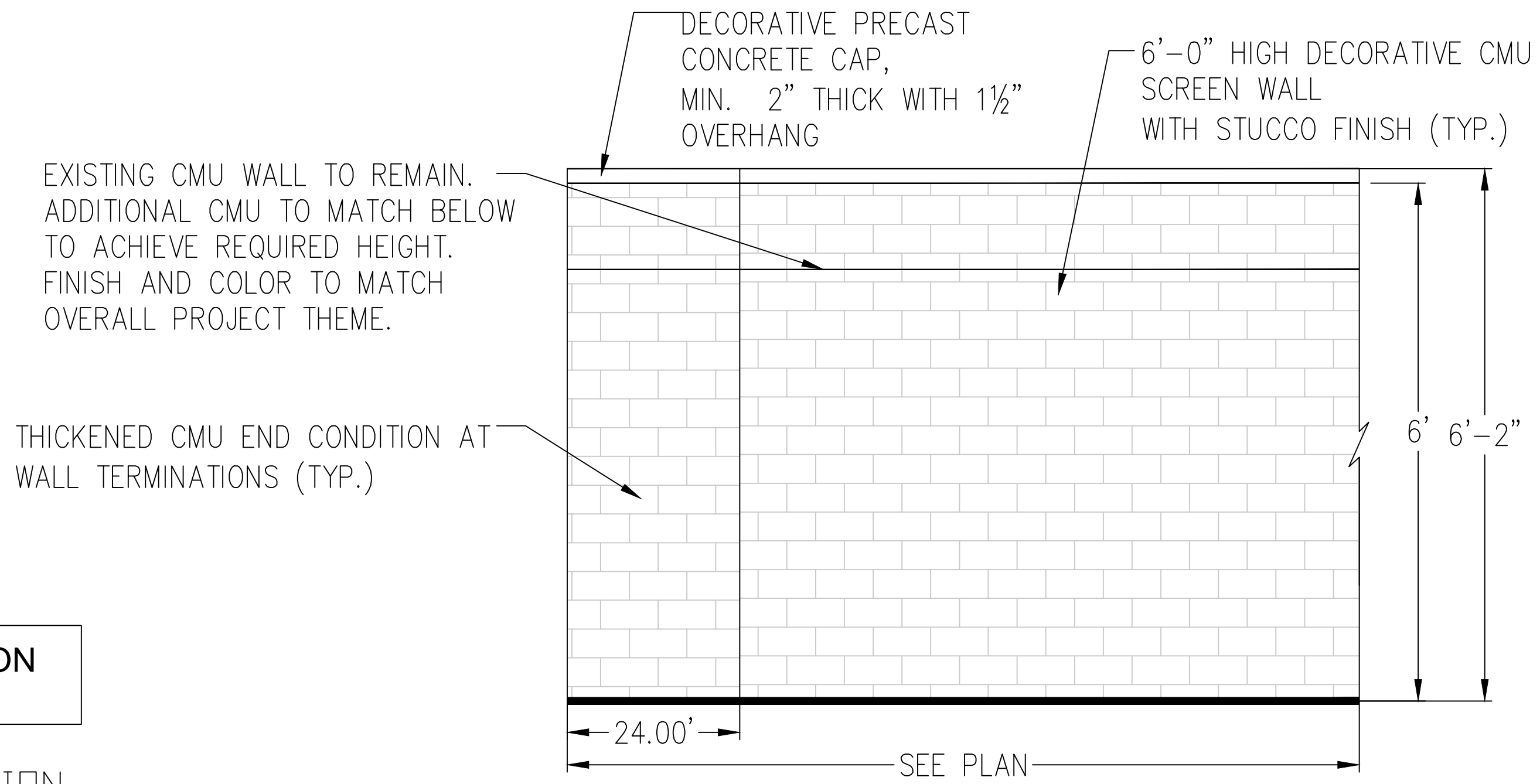
2 DECORATIVE WALL SCALE: 3/4" = 1'-0"
