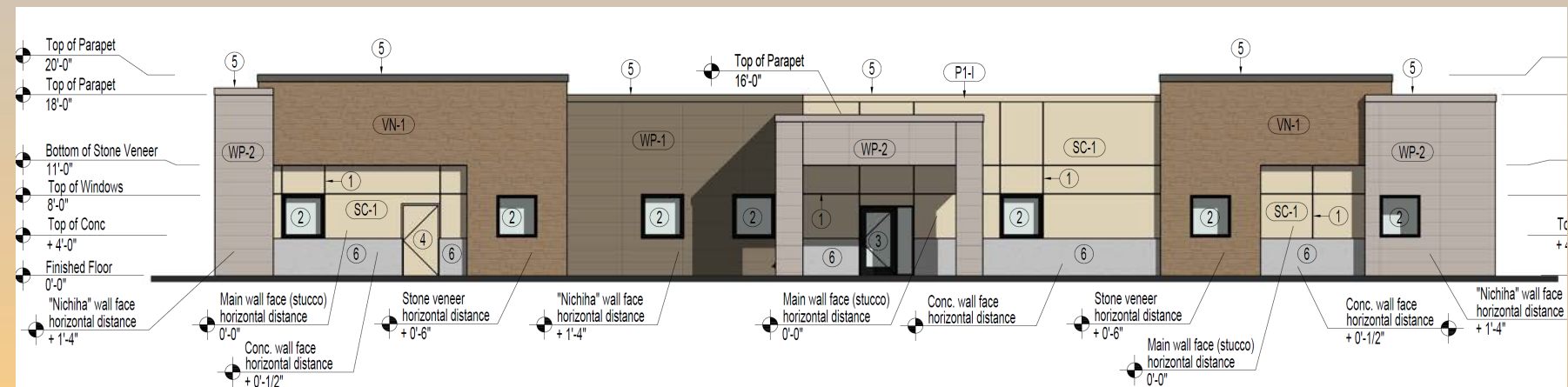
East Exterior Elevation
