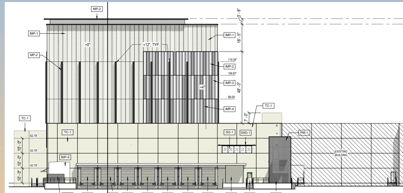
West Elevation
