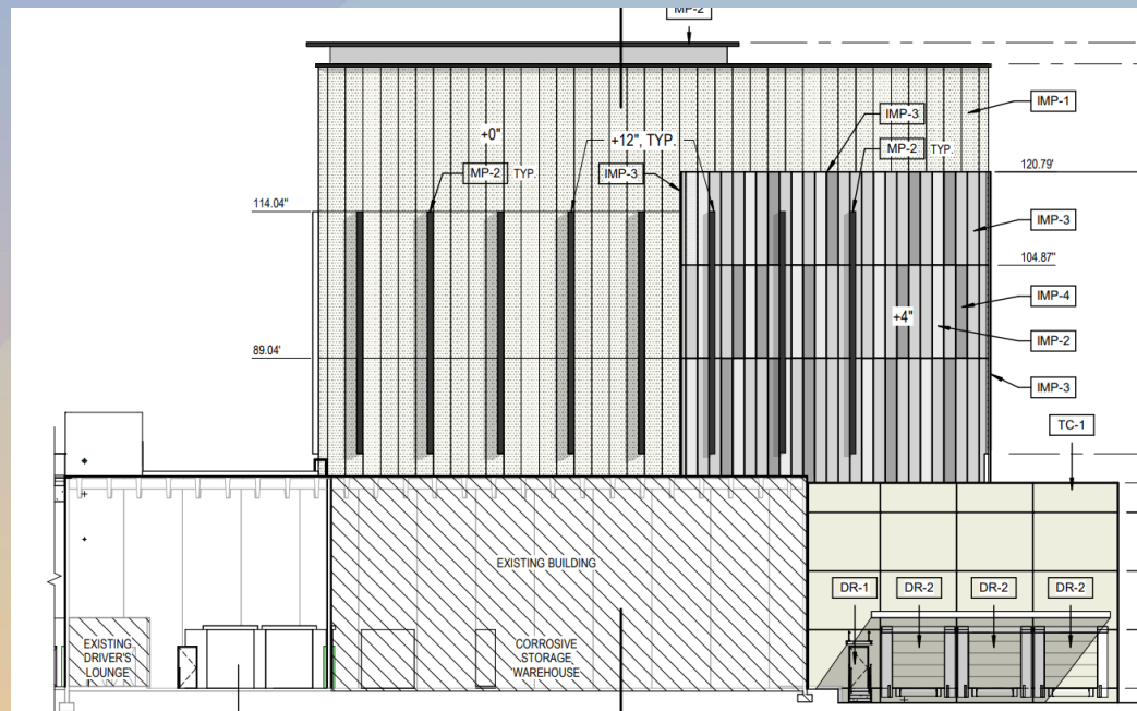
East Elevation
