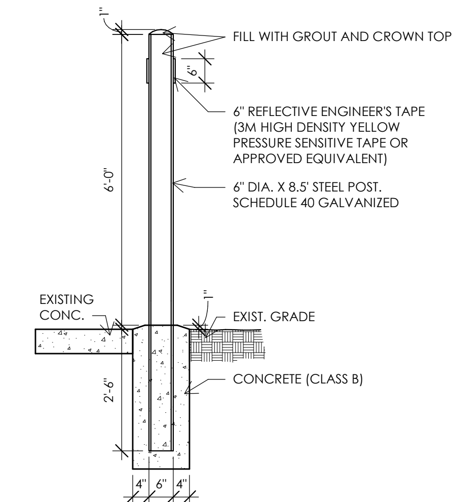
4 SAFETY POST 1/2" = 1'-0"
