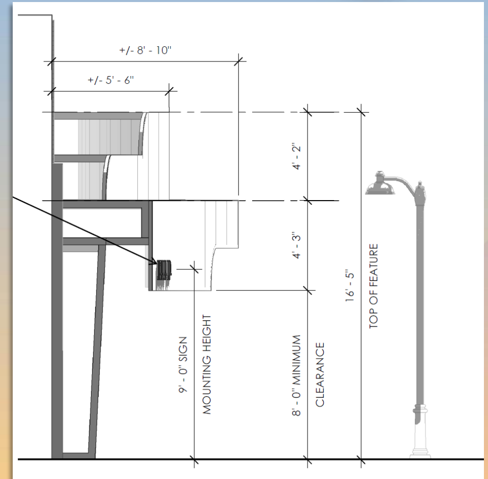
West Elevation
