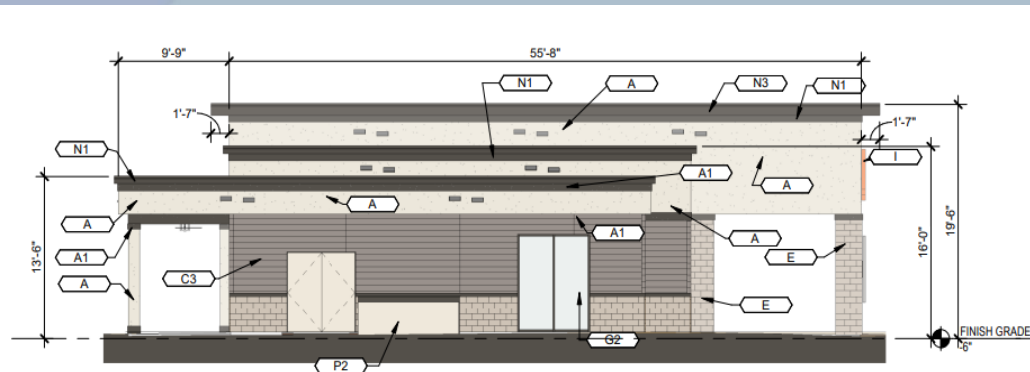
4 CLUBHOUSE - LEFT ELEVATION SCALE: 1/8" = 1'-0"
