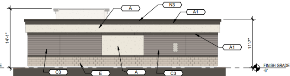
3 MAIL BUILDING - REAR ELEVATION A9 SCALE: 1/8" = 1'-0"
