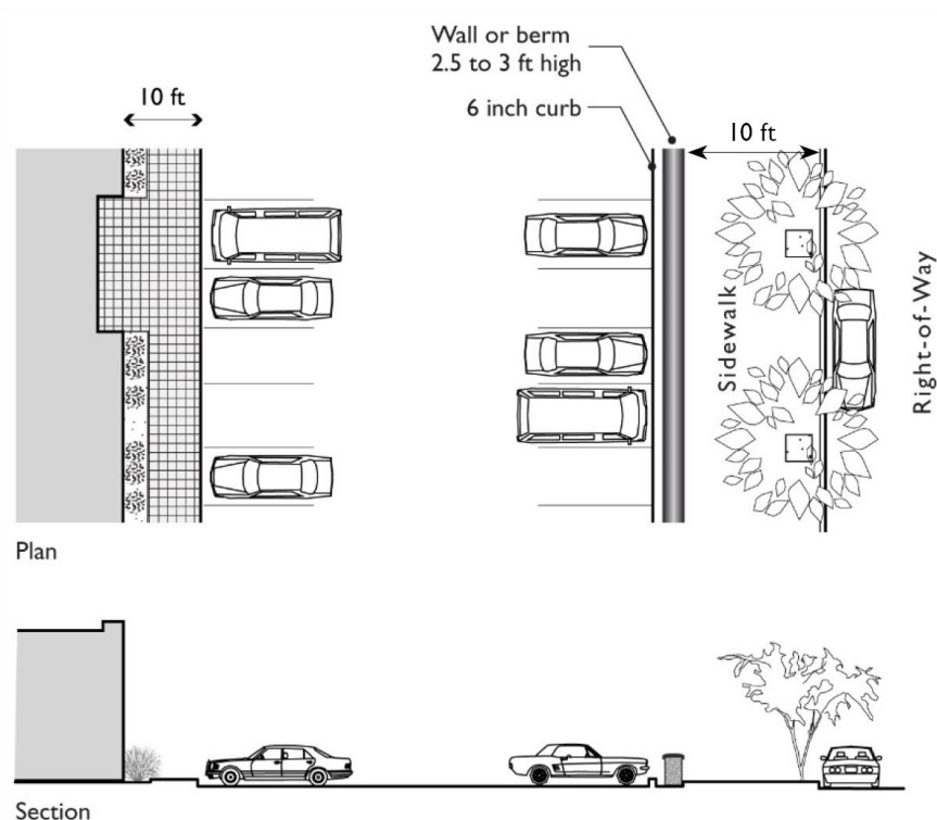
FIGURE 11-30-9.G(1): SCREENING AND SEPARATION OF PARKING AREA
