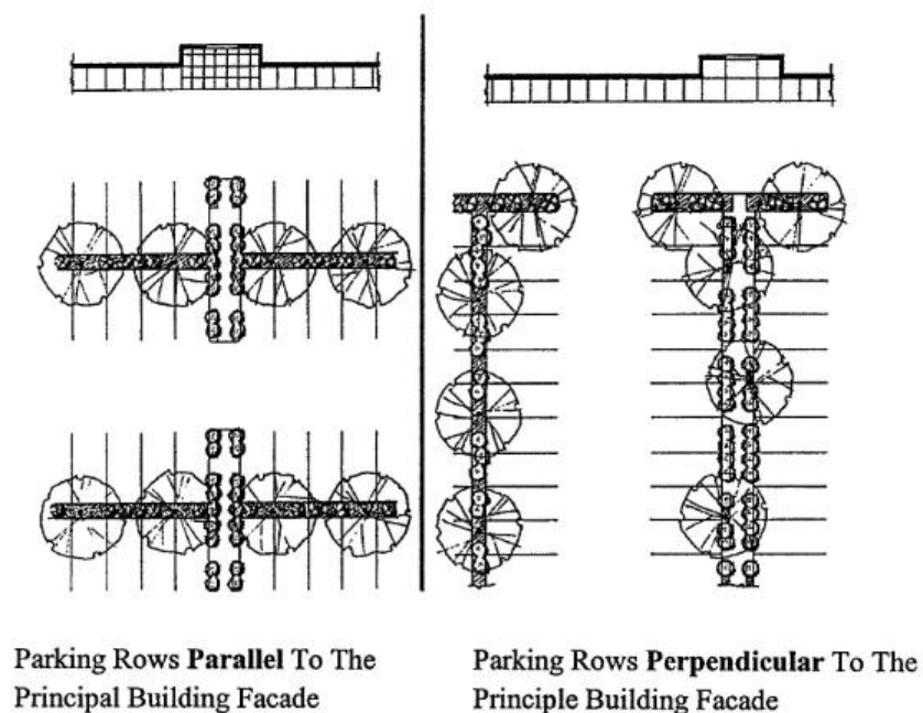
FIGURE 11-32-4.G(2): PARKING ROW ORIENTATION
