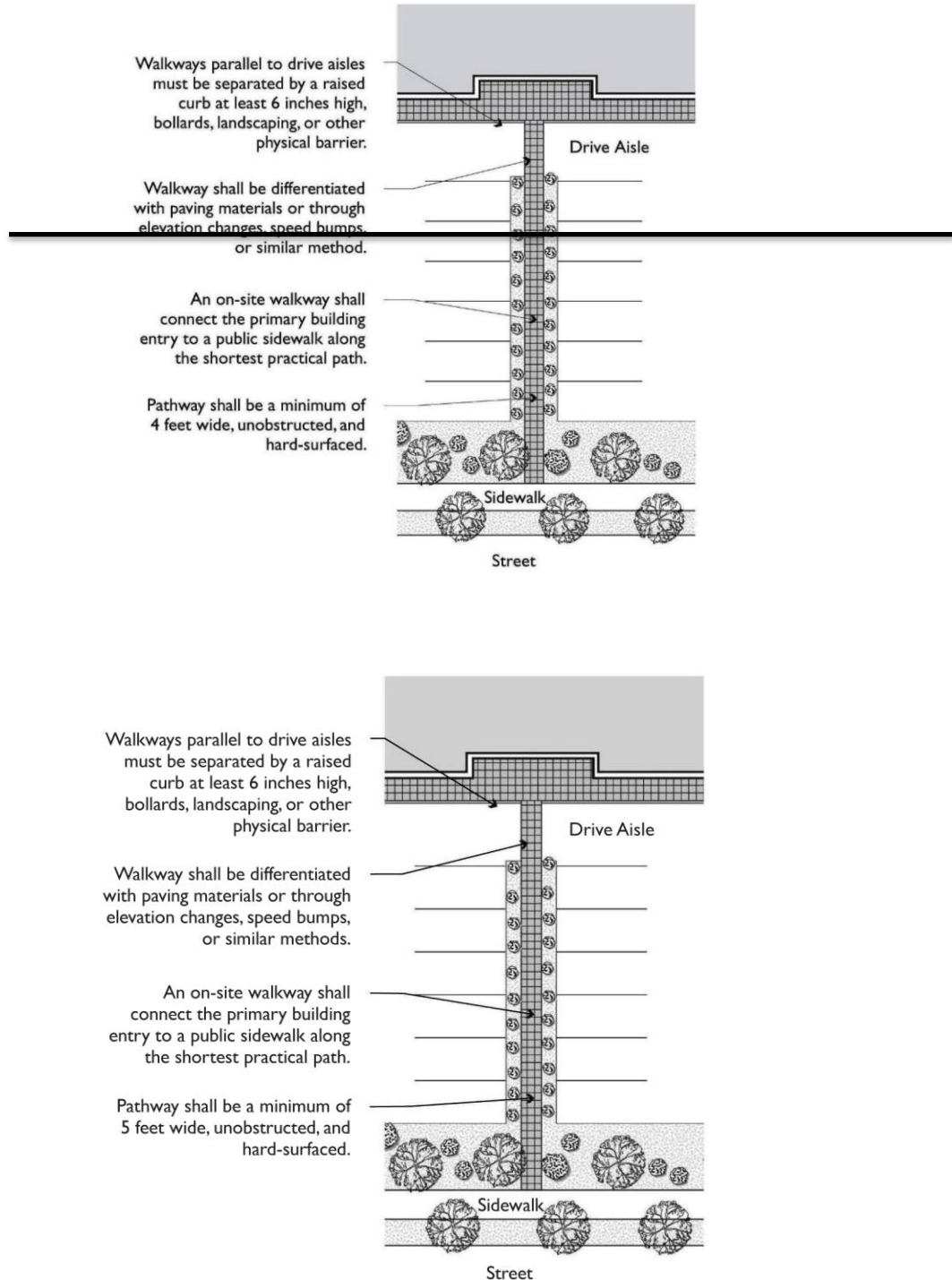
FIGURE 11-30-8.A(1): PEDESTRIAN ACCESS THROUGH PARKING AREA
