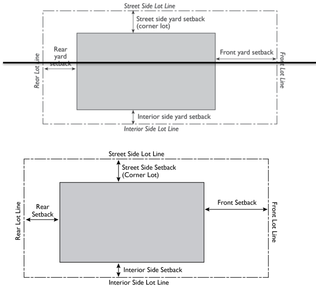
FIGURE 11-2-3.L: DETERMINING SETBACKS
