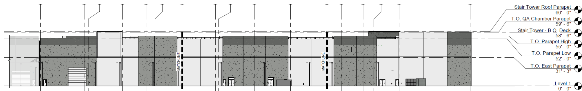
East Elevation
