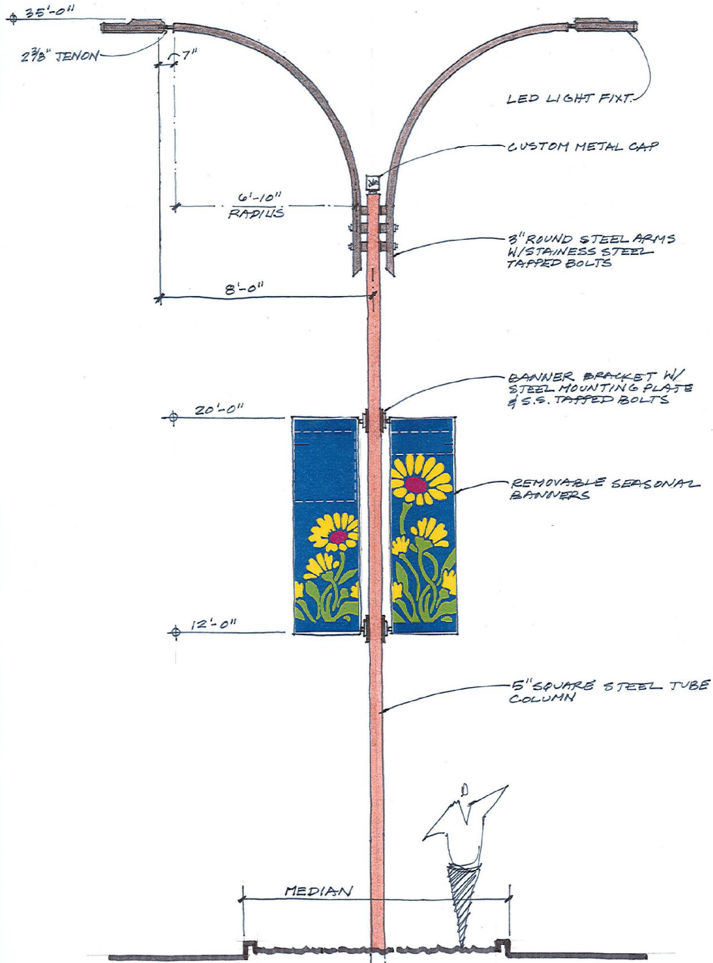
Exhibit 5.12 – Major Street Lighting – Metal Pole
