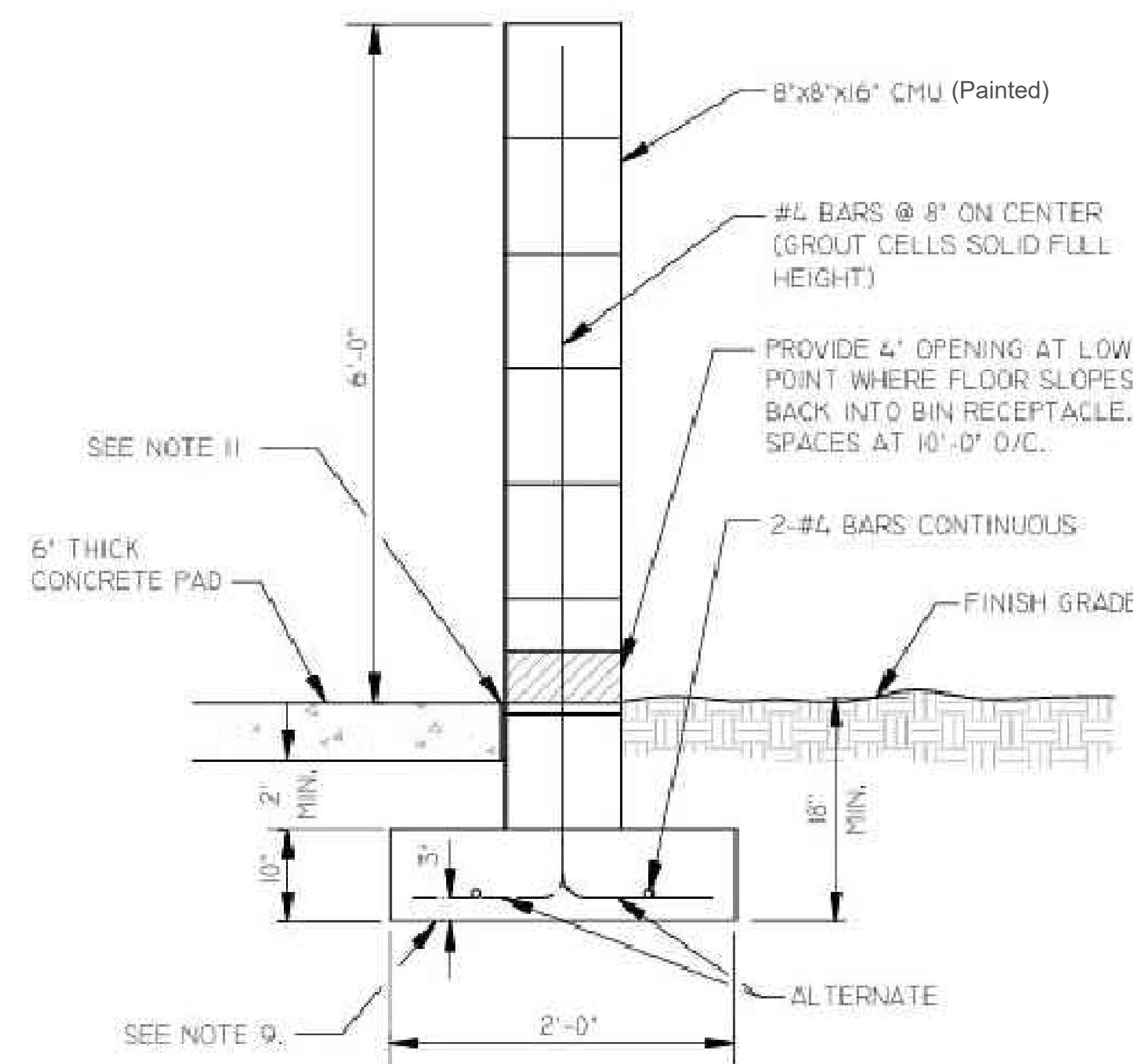
2 Trash Enclosure 6'-0" Masonry Screen Wall
