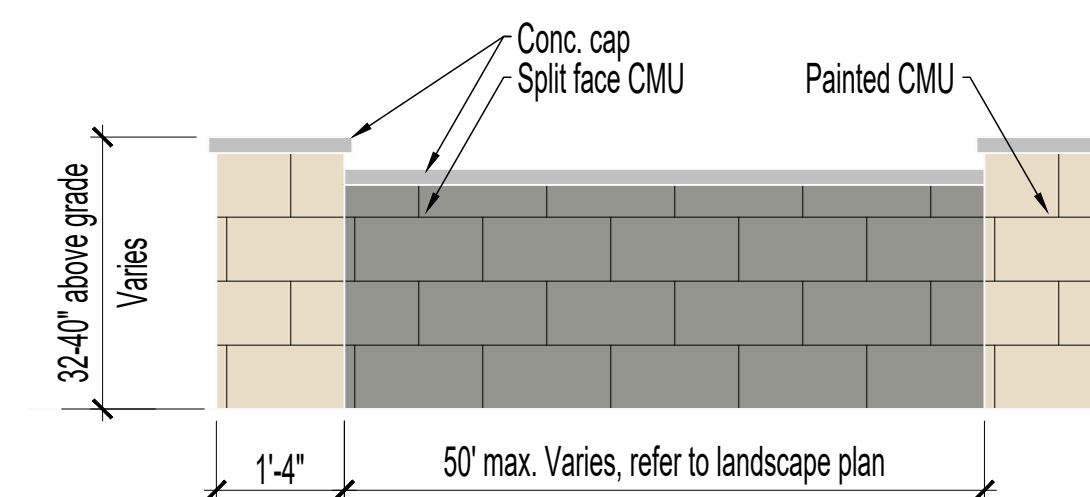
4 Typical Landscape Masonry Screen Wall
