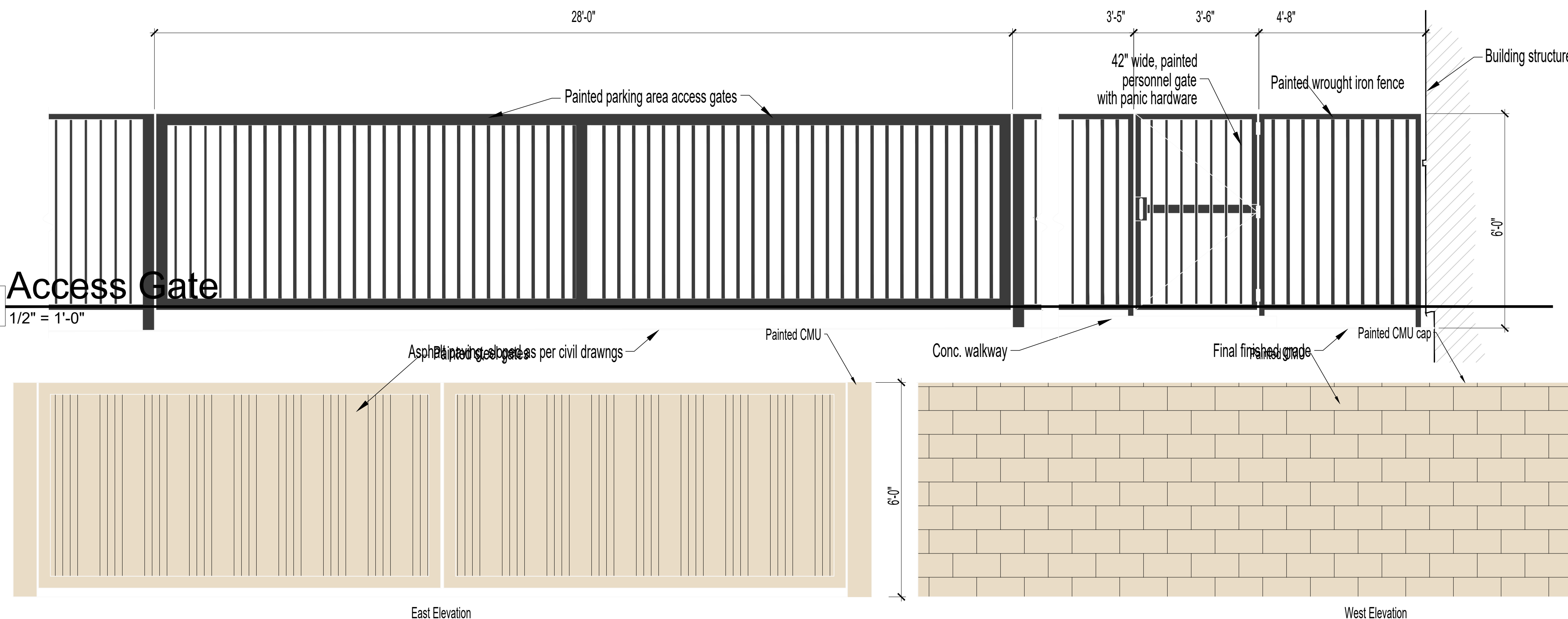
7 Trash Enclosure Exterior Elevations
