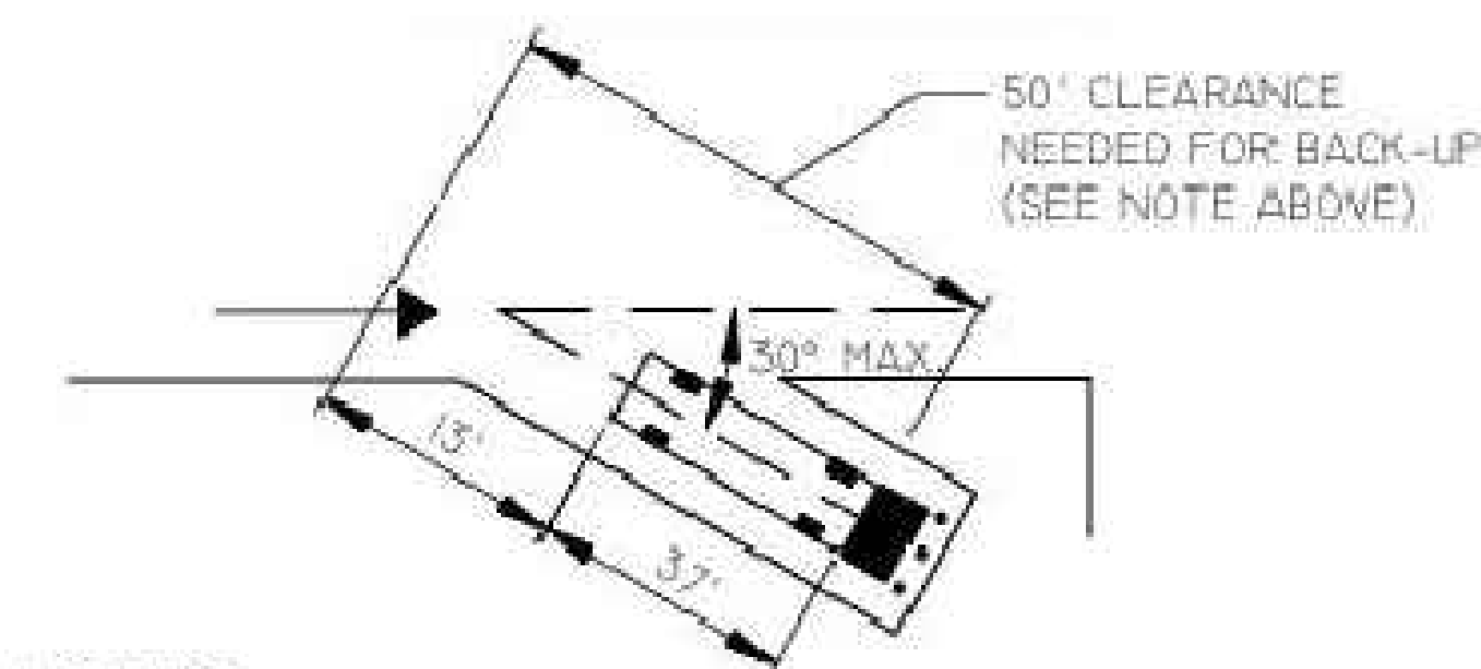
City of Mesa Standard Detail M-62.02.1
