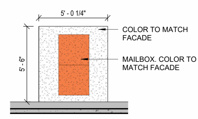
6 MAIL KIOSK 1/4" = 1'-0"
