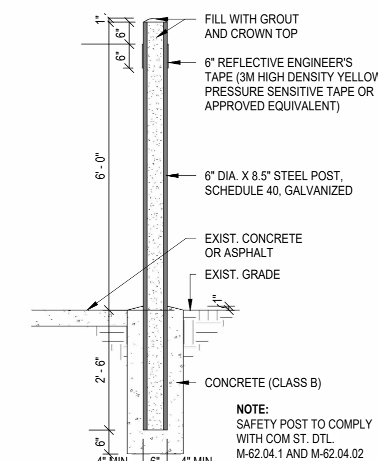
3 ENCLOSURE SAFETY POST_COM 1/2" = 1'-0"
