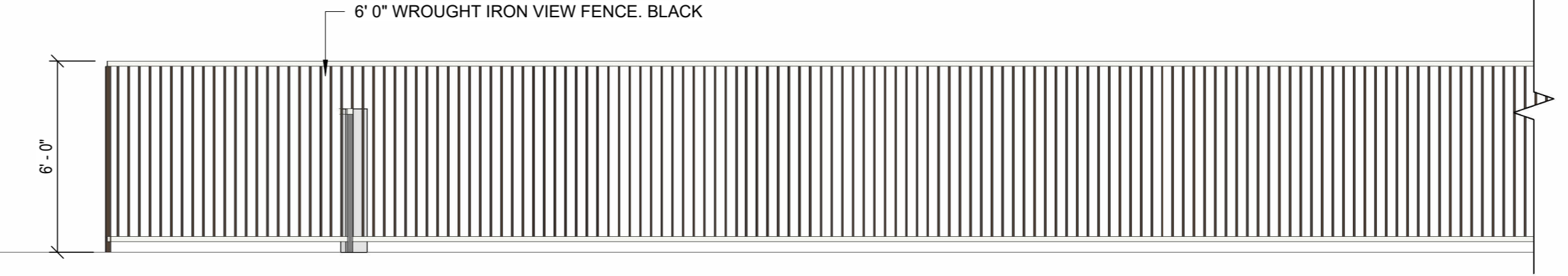
4 SITE WALL EAST 1/4" = 1'-0"
