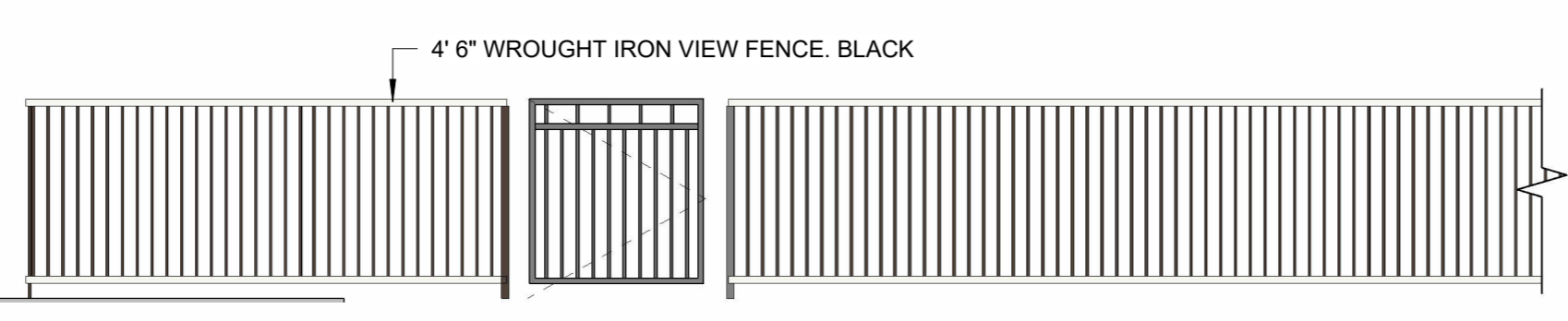
3 SITE WALL WEST 1/4" = 1'-0"
