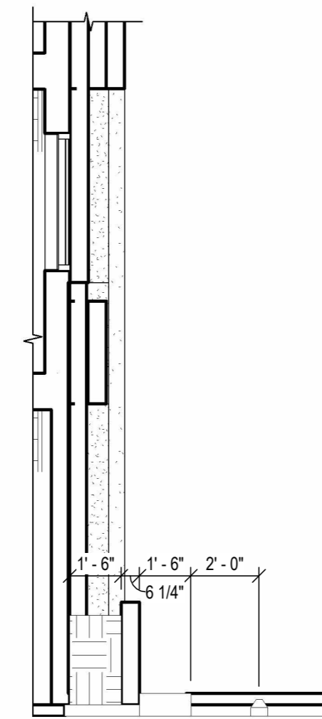
7 PLANTER FOUNDATION 1/4" = 1'-0"
