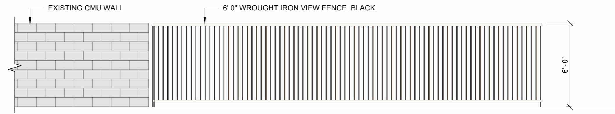
2 SITE WALL NORTH 1/4" = 1'-0"
