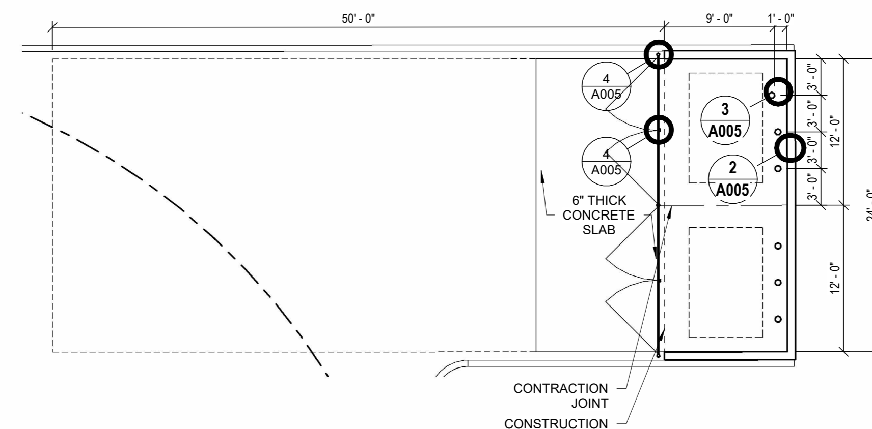
1 ENLARGED SOLID WASTE 1/8" = 1'-0"
