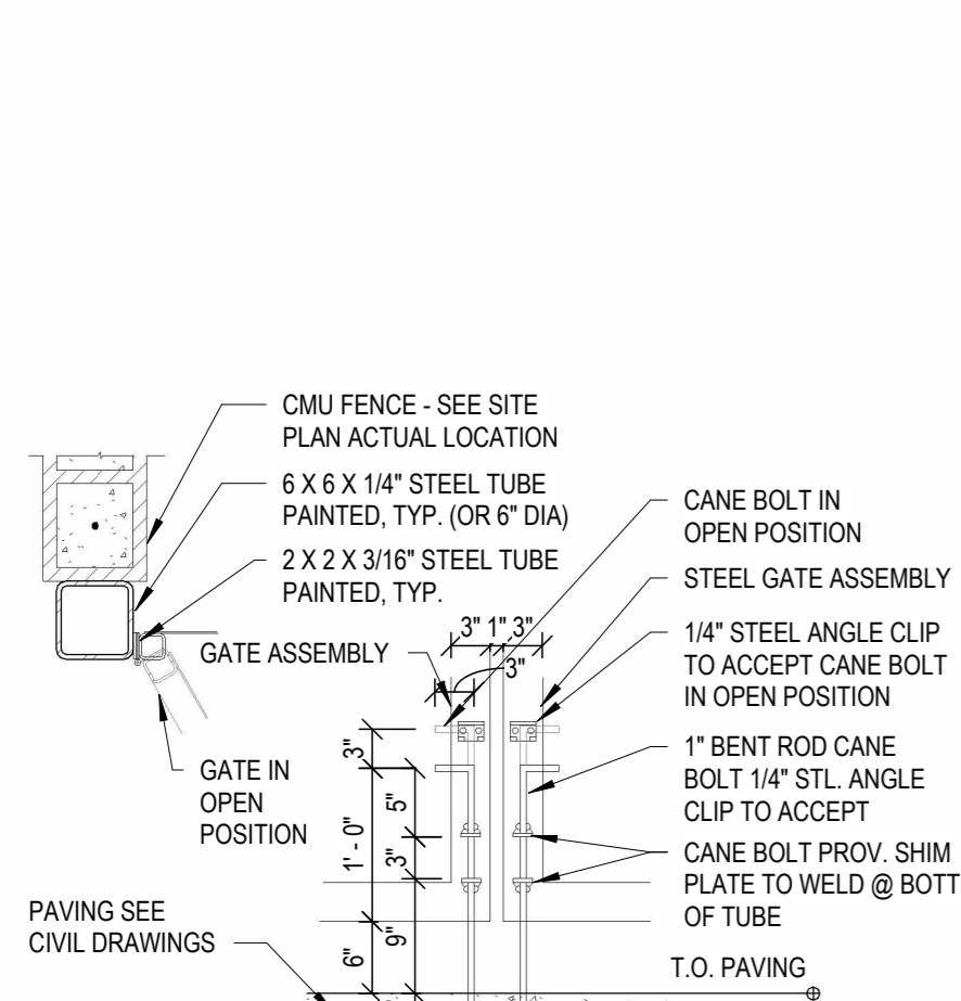
4 SITE - TRASH ENCLOSURE GATE DETAIL 3/4" = 1'-0"
