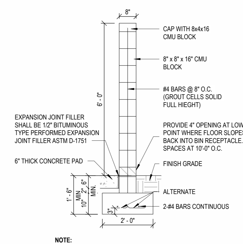
2 ENCLOSURE SCREEN WALL_COM 1/2" = 1'-0"
