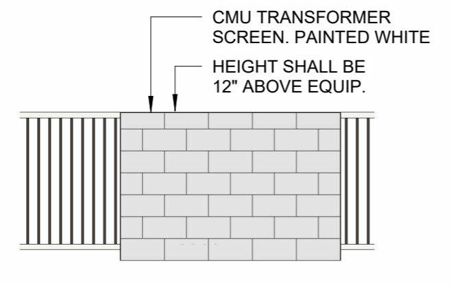
5 MECH. EQUIP. SCREEN WALL 1/4" = 1'-0"
