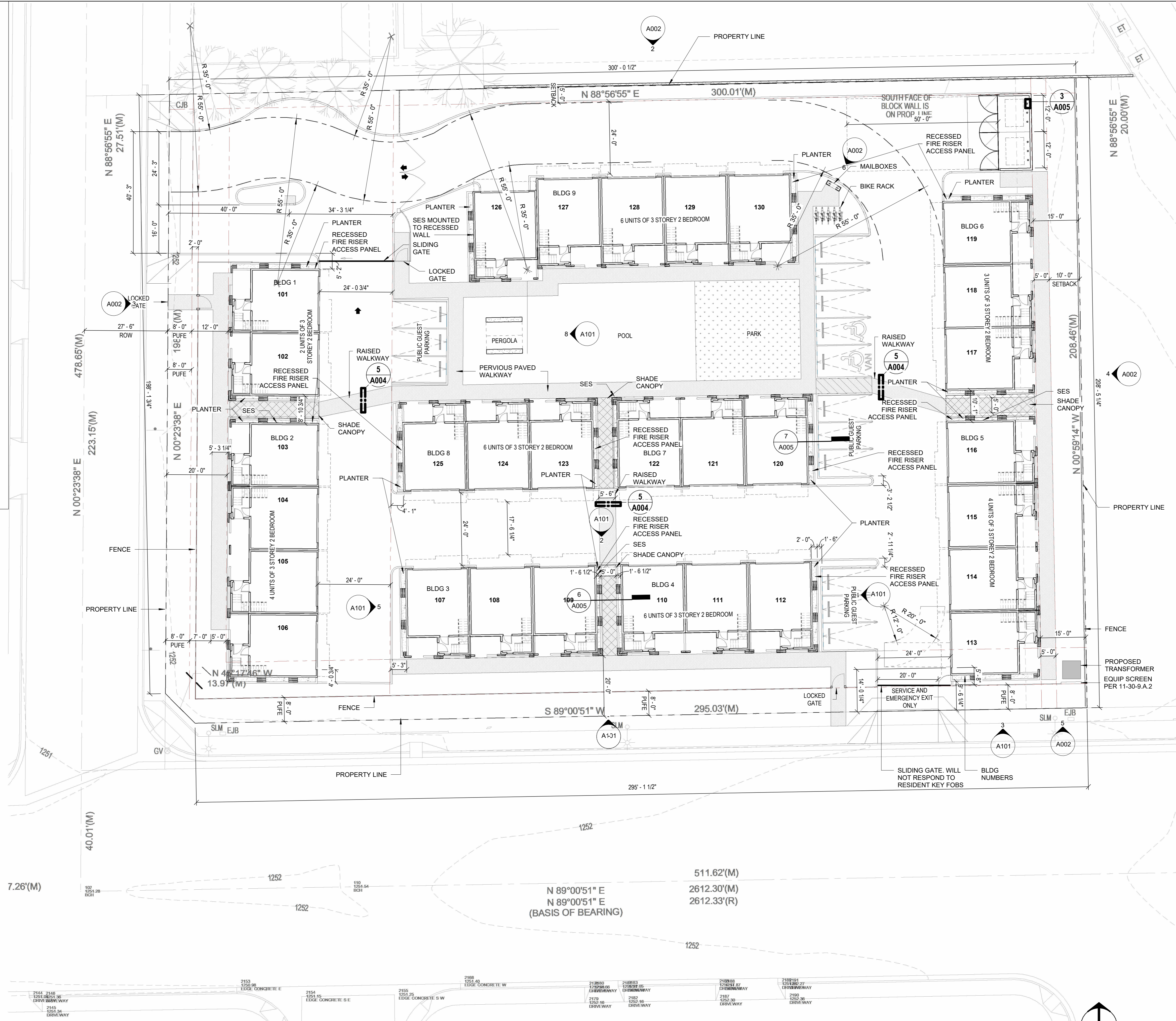
1 SITE PLAN 1/16" = 1'-0"
