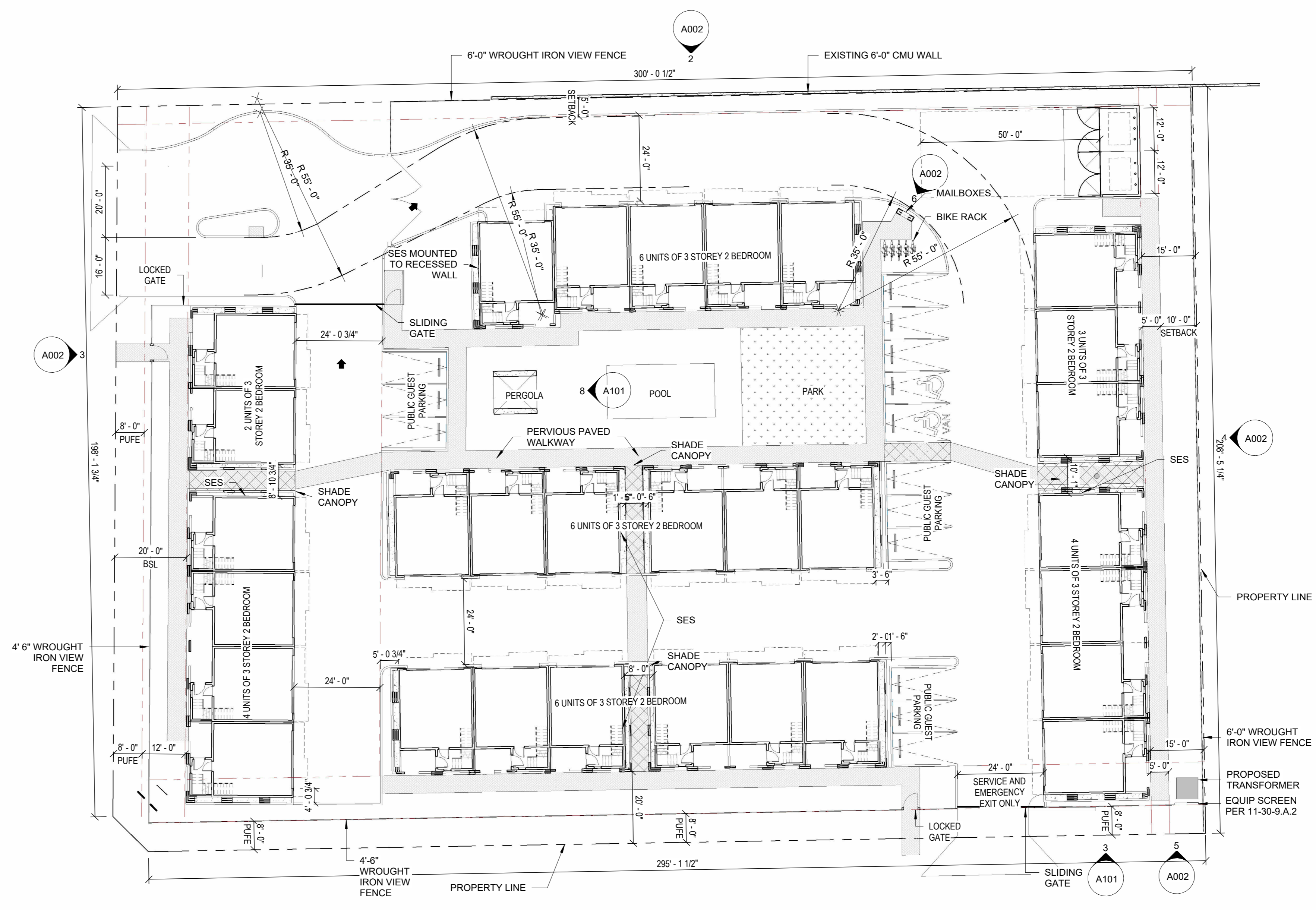
1 SITE WALL PLAN 1" = 20'-0"
