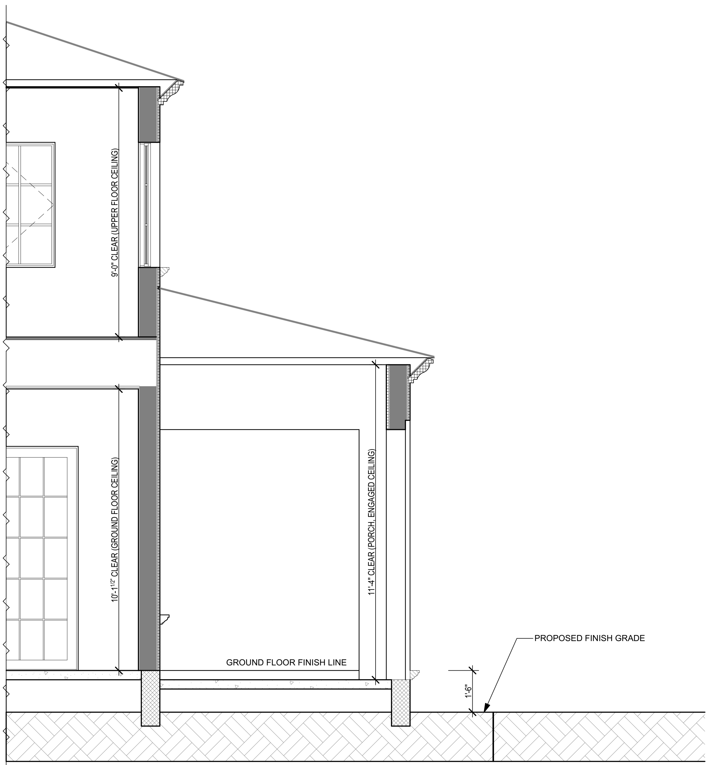
A TYPICAL BUILDING SECTION SCALE: 1/2" = 1'-0" 0 1' 2' 4'
