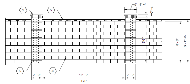
PRIMARY SITE WALL ELEVATION 1/4" = 1'-0"
