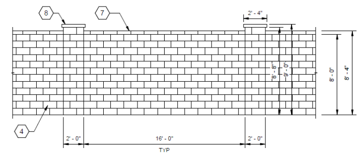
SECONDARY SITE WALL ELEVATION 1/4" = 1'-0"
