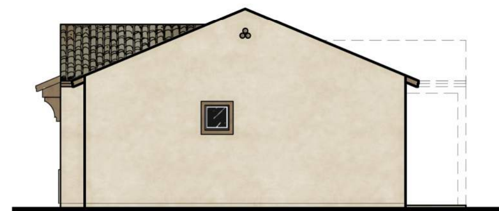
Right Elevation Elevation A 1/8" = 1'-0"
