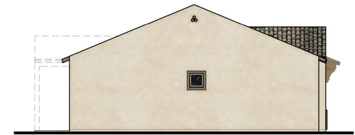
Left Elevation Elevation A 1/8" = 1'-0"
