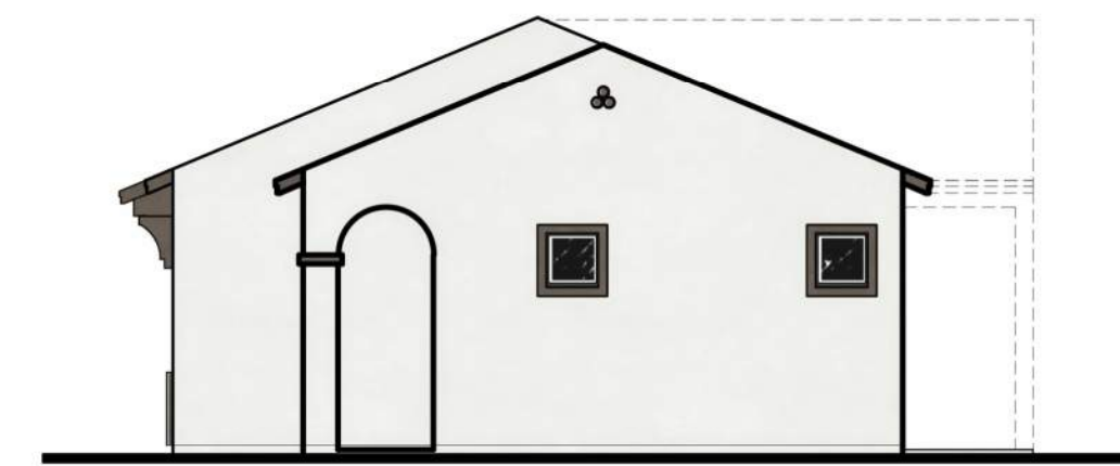
Right Elevation Elevation A 1/8" = 1'-0"
