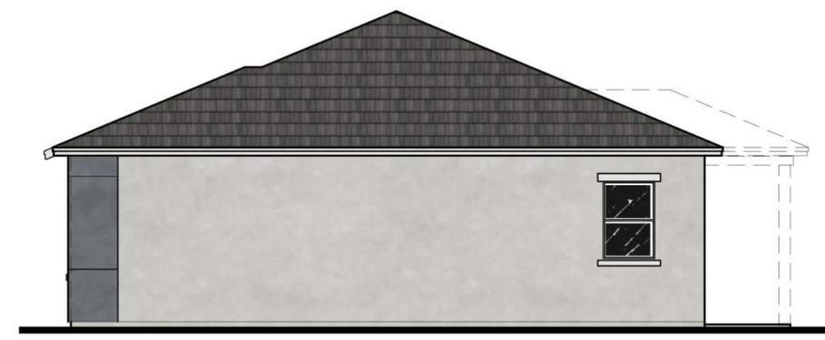
Right Elevation Elevation B 1/8" = 1'-0"
