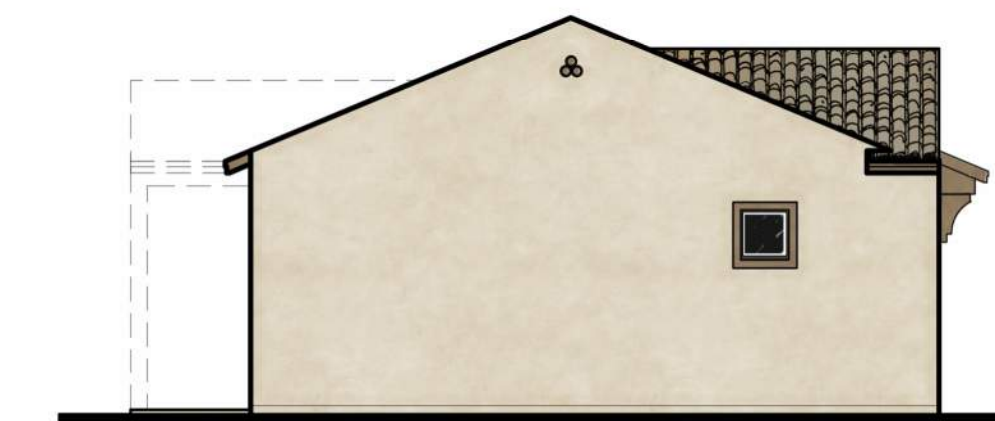
Left Elevation Elevation A 1/8" = 1'-0"
