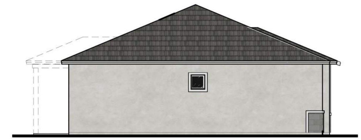
Left Elevation Elevation B 1/8" = 1'-0"
