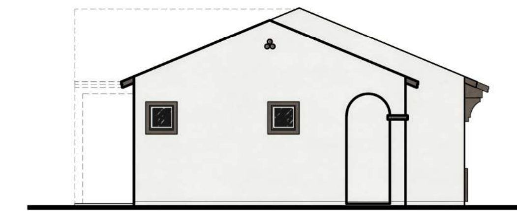
Left Elevation Elevation A 1/8" = 1'-0"
