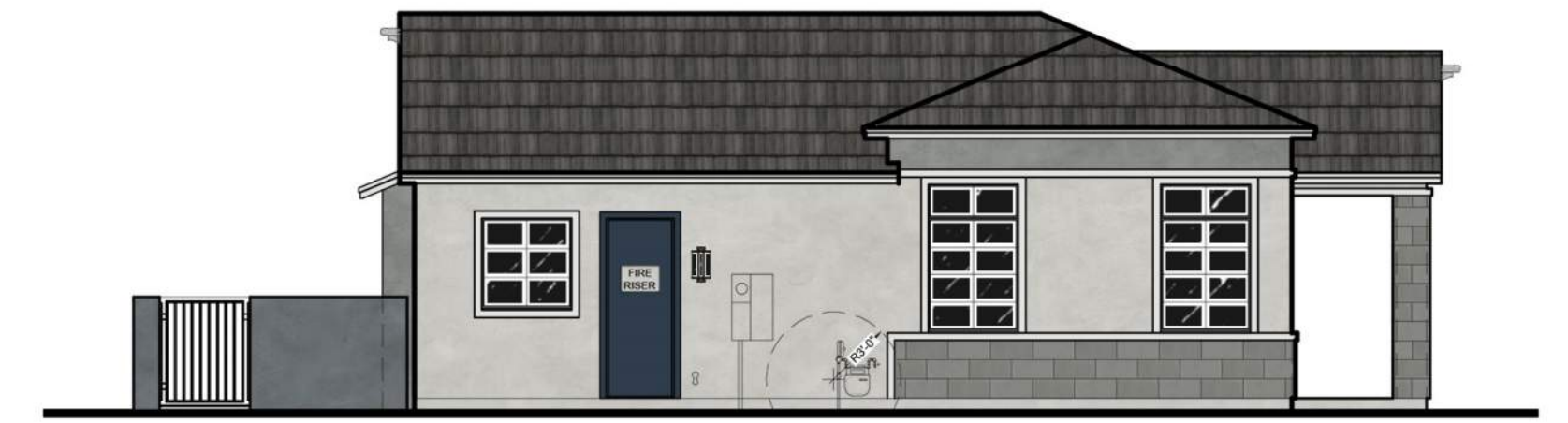
Left Elevation Elevation A 1/8" = 1'-0"
